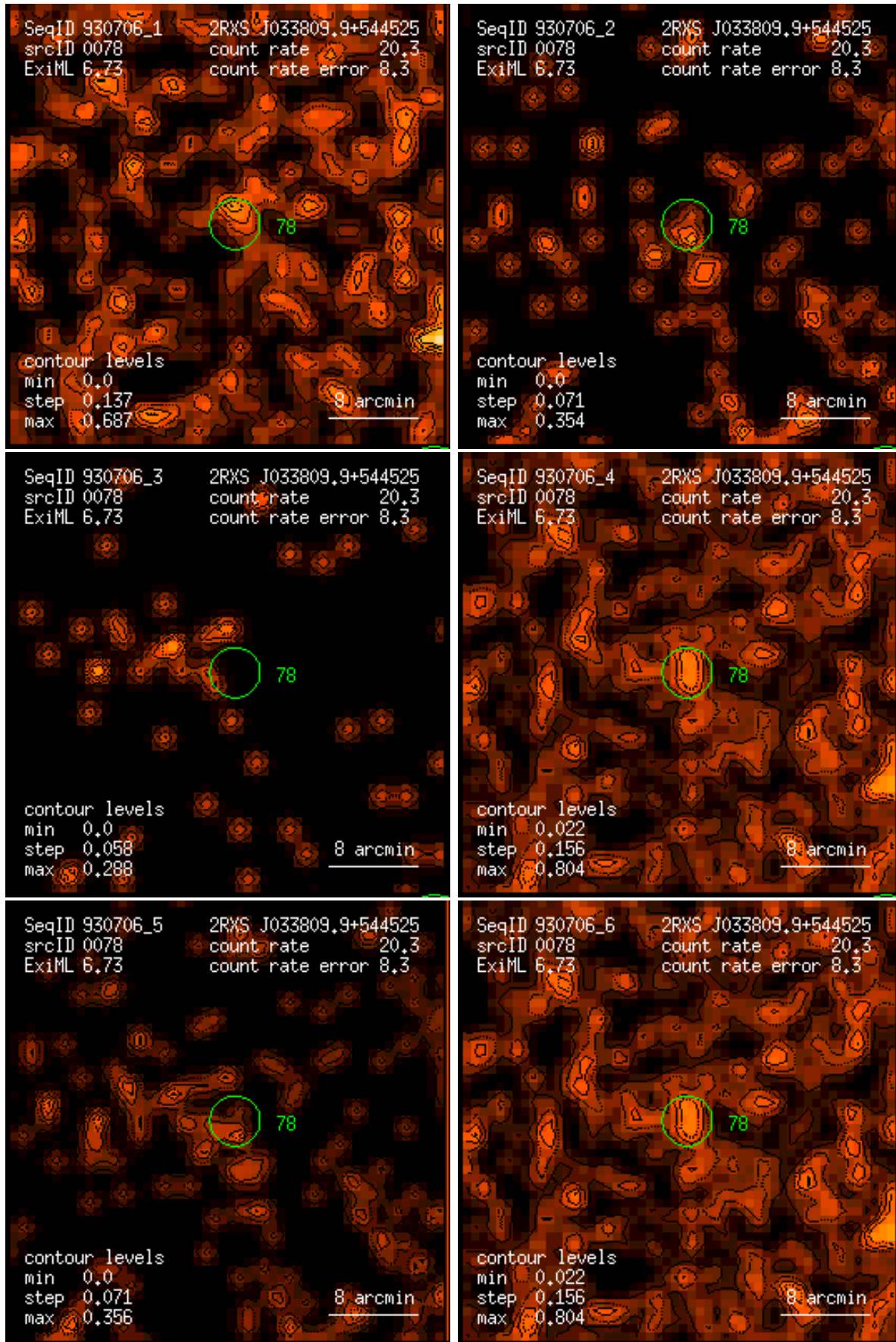
Figure 78: RASS 930706: detection 0078: band rate images, Gaussian filter: (1) PSPC channels 11 – 41, (2) 52 – 90, (3) 91 – 201, (4) 11 – 235, (5) 52 – 201, (6) 11 – 201. Broad band rates in counts/ks. Band rate contour levels in counts/ks/arcmin 2 .
