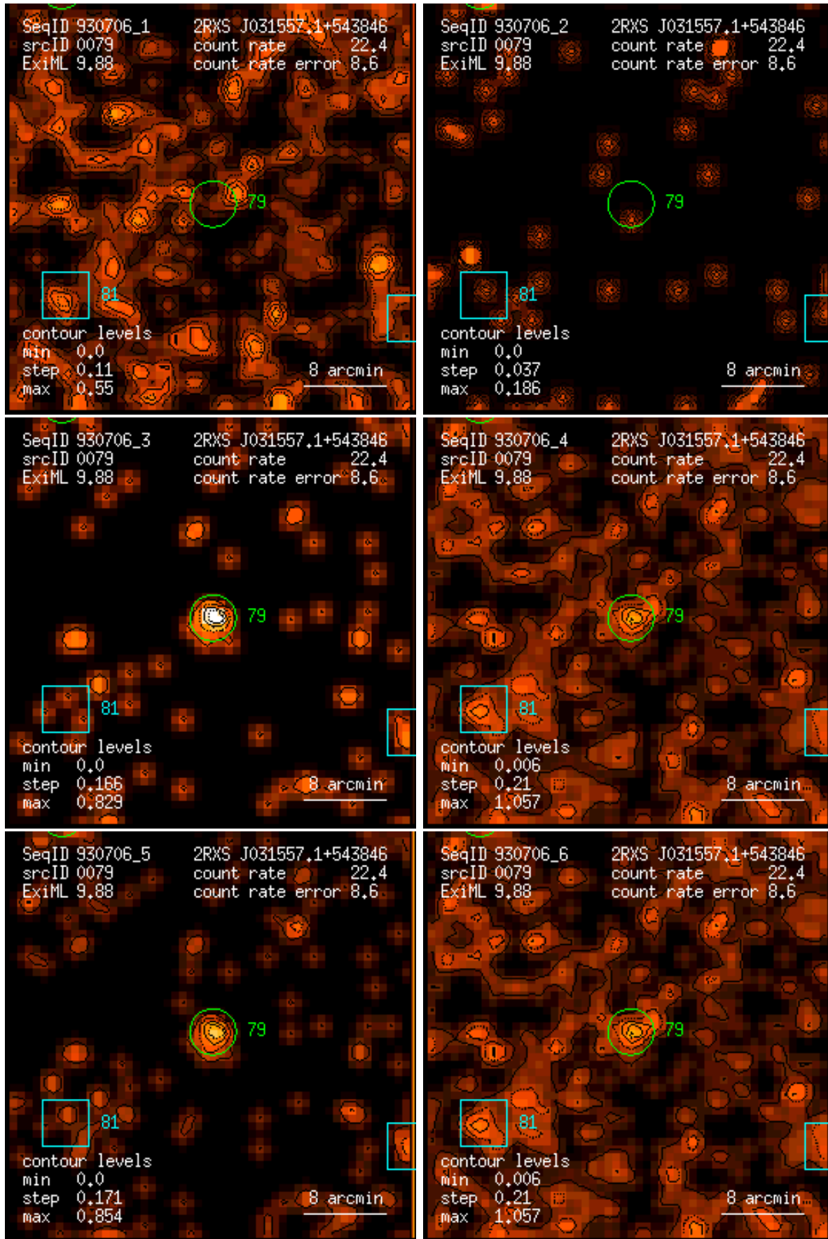
Figure 79: RASS 930706: detection 0079: band rate images, Gaussian filter: (1) PSPC channels 11 – 41, (2) 52 – 90, (3) 91 – 201, (4) 11 – 235, (5) 52 – 201, (6) 11 – 201. Broad band rates in counts/ks. Band rate contour levels in counts/ks/arcmin 2 .
