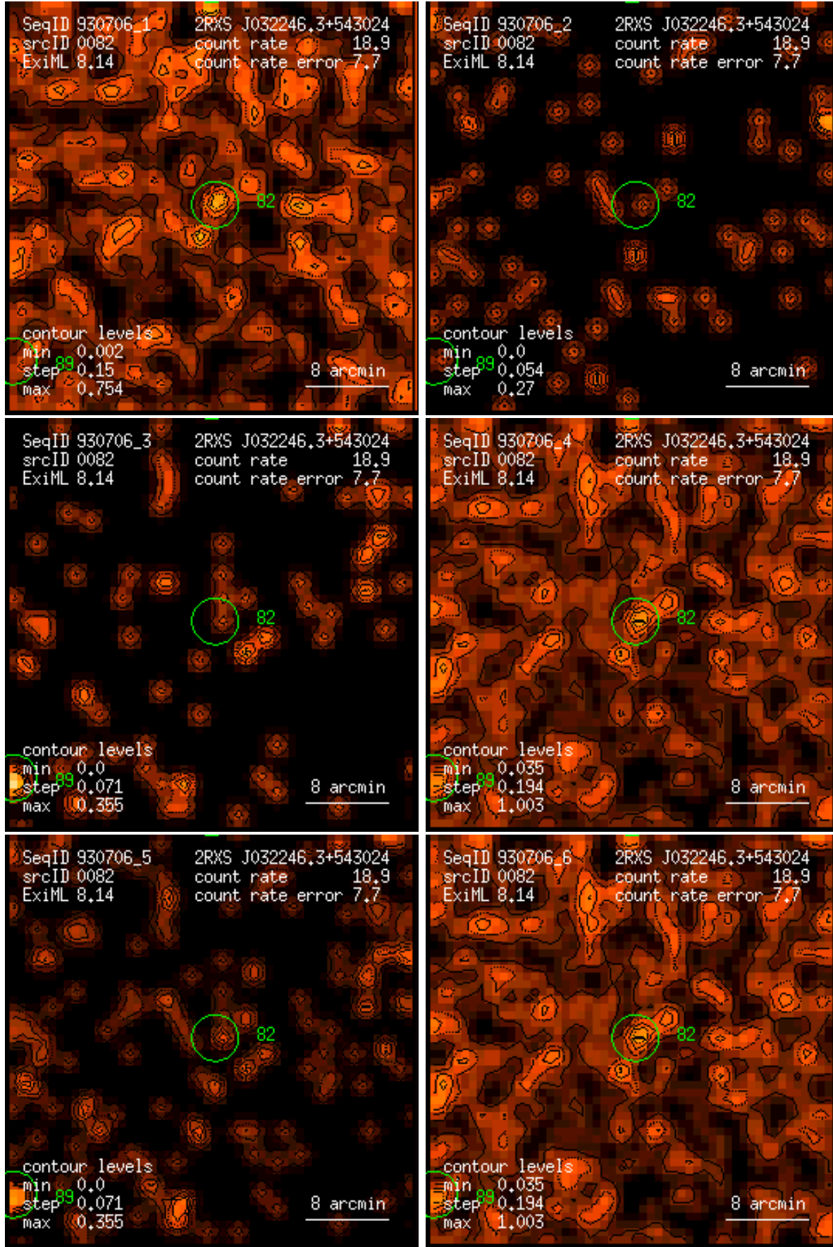
Figure 82: RASS 930706: detection 0082: band rate images, Gaussian filter: (1) PSPC channels 11 – 41, (2) 52 – 90, (3) 91 – 201, (4) 11 – 235, (5) 52 – 201, (6) 11 – 201. Broad band rates in counts/ks. Band rate contour levels in counts/ks/arcmin 2 .
