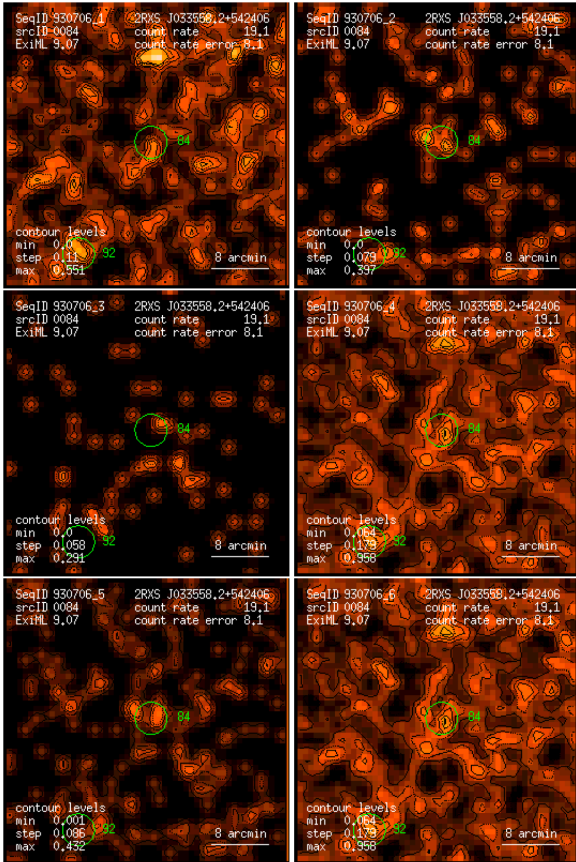
Figure 84: RASS 930706: detection 0084: band rate images, Gaussian filter: (1) PSPC channels 11 – 41, (2) 52 – 90, (3) 91 – 201, (4) 11 – 235, (5) 52 – 201, (6) 11 – 201. Broad band rates in counts/ks. Band rate contour levels in counts/ks/arcmin 2 .
