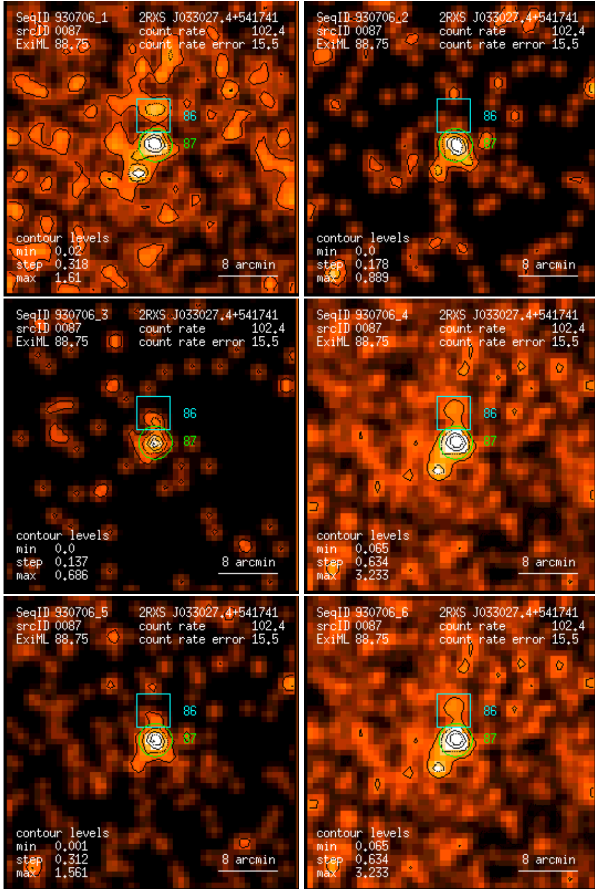
Figure 87: RASS 930706: detection 0087: band rate images, Gaussian filter: (1) PSPC channels 11 – 41, (2) 52 – 90, (3) 91 – 201, (4) 11 – 235, (5) 52 – 201, (6) 11 – 201. Broad band rates in counts/ks. Band rate contour levels in counts/ks/arcmin 2 .
