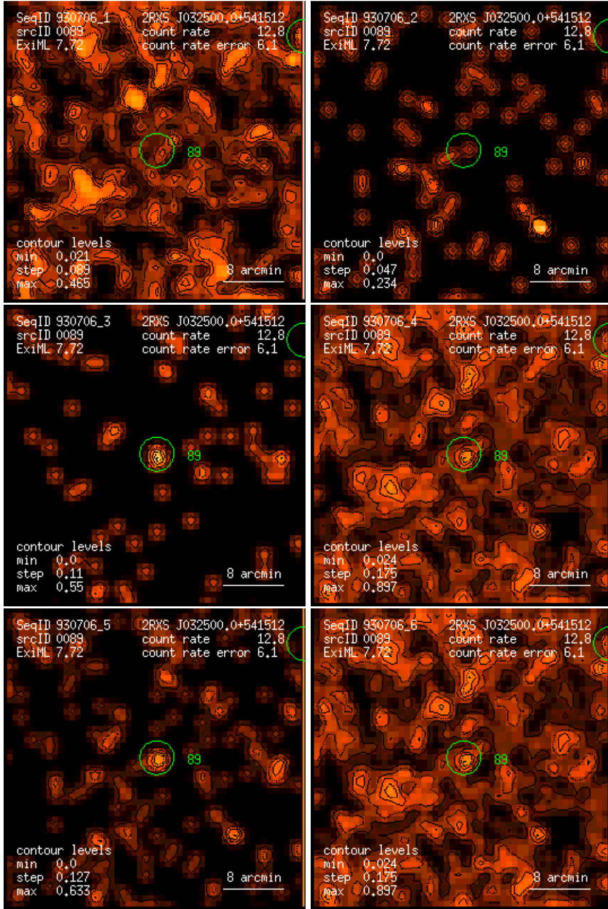
Figure 89: RASS 930706: detection 0089: band rate images, Gaussian filter: (1) PSPC channels 11 – 41, (2) 52 – 90, (3) 91 – 201, (4) 11 – 235, (5) 52 – 201, (6) 11 – 201. Broad band rates in counts/ks. Band rate contour levels in counts/ks/arcmin 2 .
