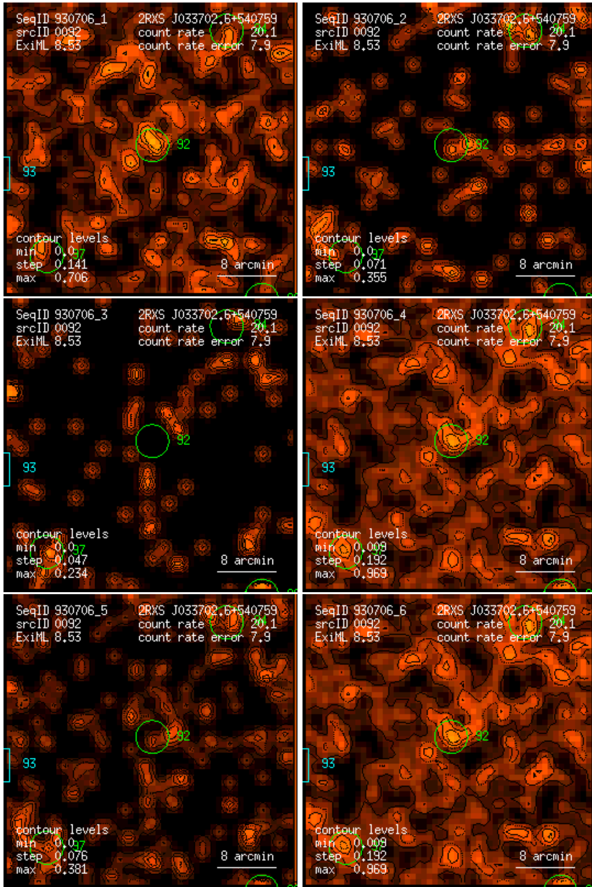
Figure 92: RASS 930706: detection 0092: band rate images, Gaussian filter: (1) PSPC channels 11 – 41, (2) 52 – 90, (3) 91 – 201, (4) 11 – 235, (5) 52 – 201, (6) 11 – 201. Broad band rates in counts/ks. Band rate contour levels in counts/ks/arcmin 2 .
