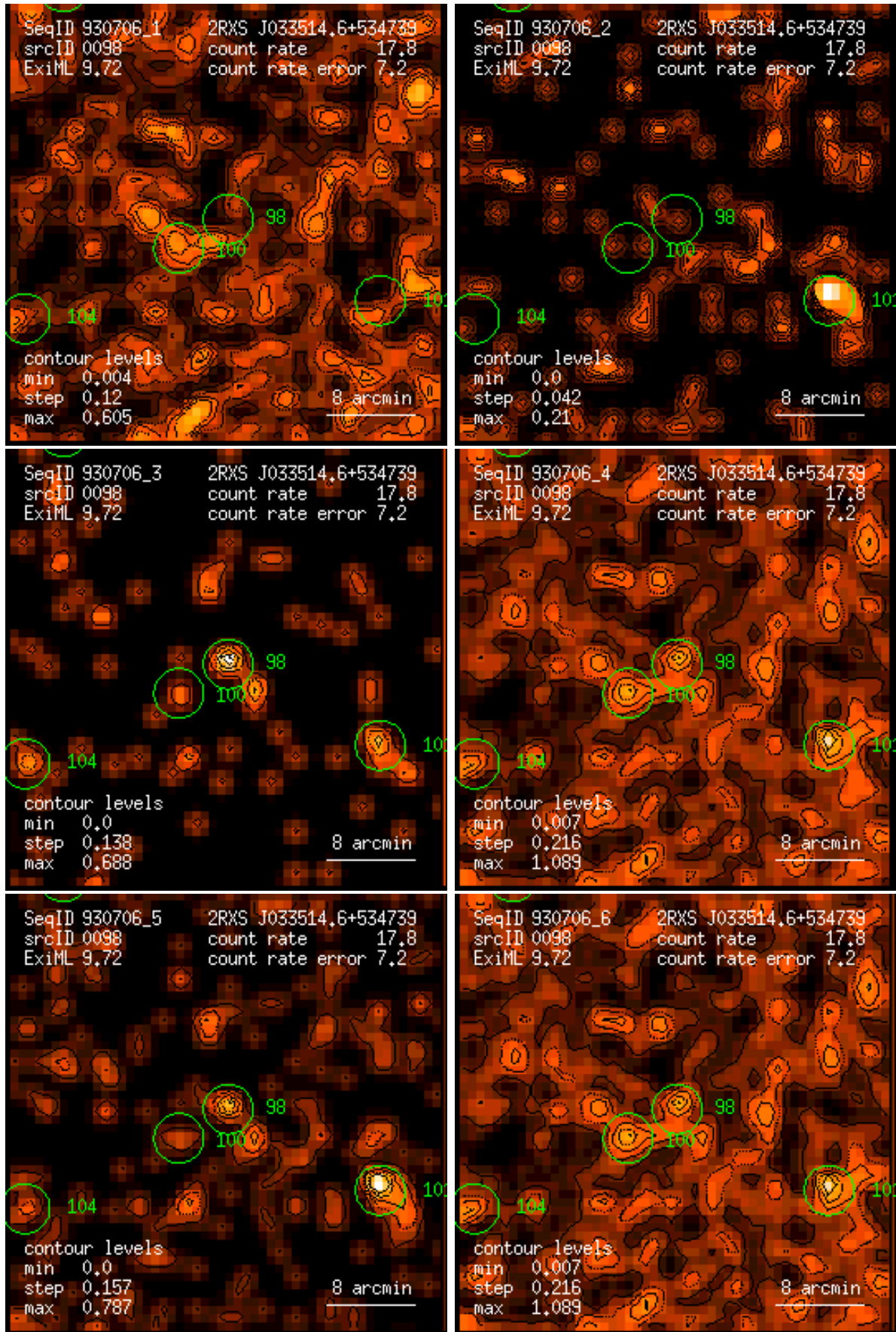
Figure 98: RASS 930706: detection 0098: band rate images, Gaussian filter: (1) PSPC channels 11 – 41, (2) 52 – 90, (3) 91 – 201, (4) 11 – 235, (5) 52 – 201, (6) 11 – 201. Broad band rates in counts/ks. Band rate contour levels in counts/ks/arcmin 2 .
