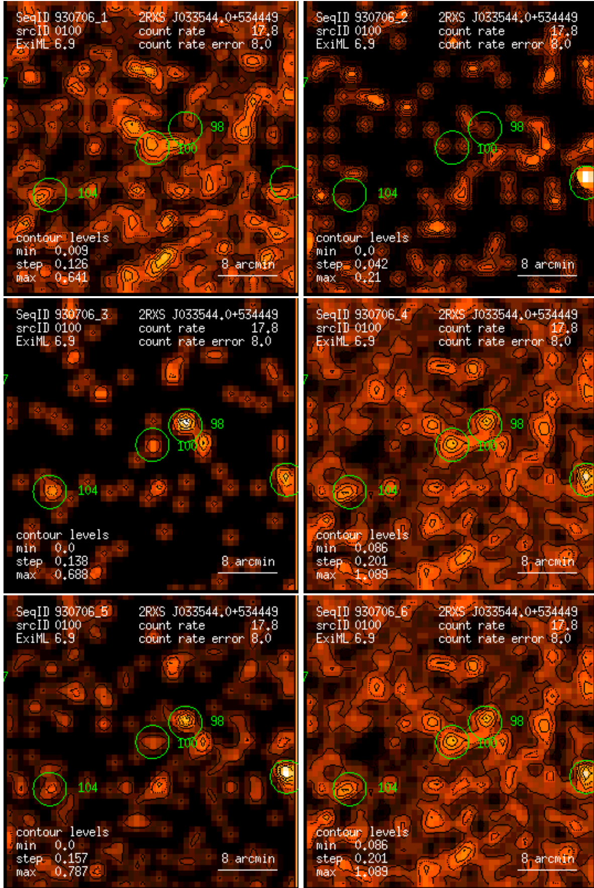
Figure 100: RASS 930706: detection 0100: band rate images, Gaussian filter: (1) PSPC channels 11 – 41, (2) 52 – 90, (3) 91 – 201, (4) 11 – 235, (5) 52 – 201, (6) 11 – 201. Broad band rates in counts/ks. Band rate contour levels in counts/ks/arcmin 2 .
