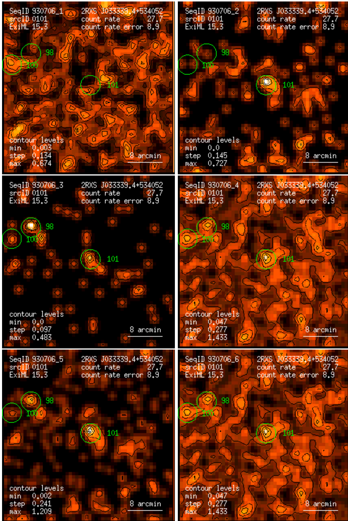
Figure 101: RASS 930706: detection 0101: band rate images, Gaussian filter: (1) PSPC channels 11 – 41, (2) 52 – 90, (3) 91 – 201, (4) 11 – 235, (5) 52 – 201, (6) 11 – 201. Broad band rates in counts/ks. Band rate contour levels in counts/ks/arcmin 2 .
