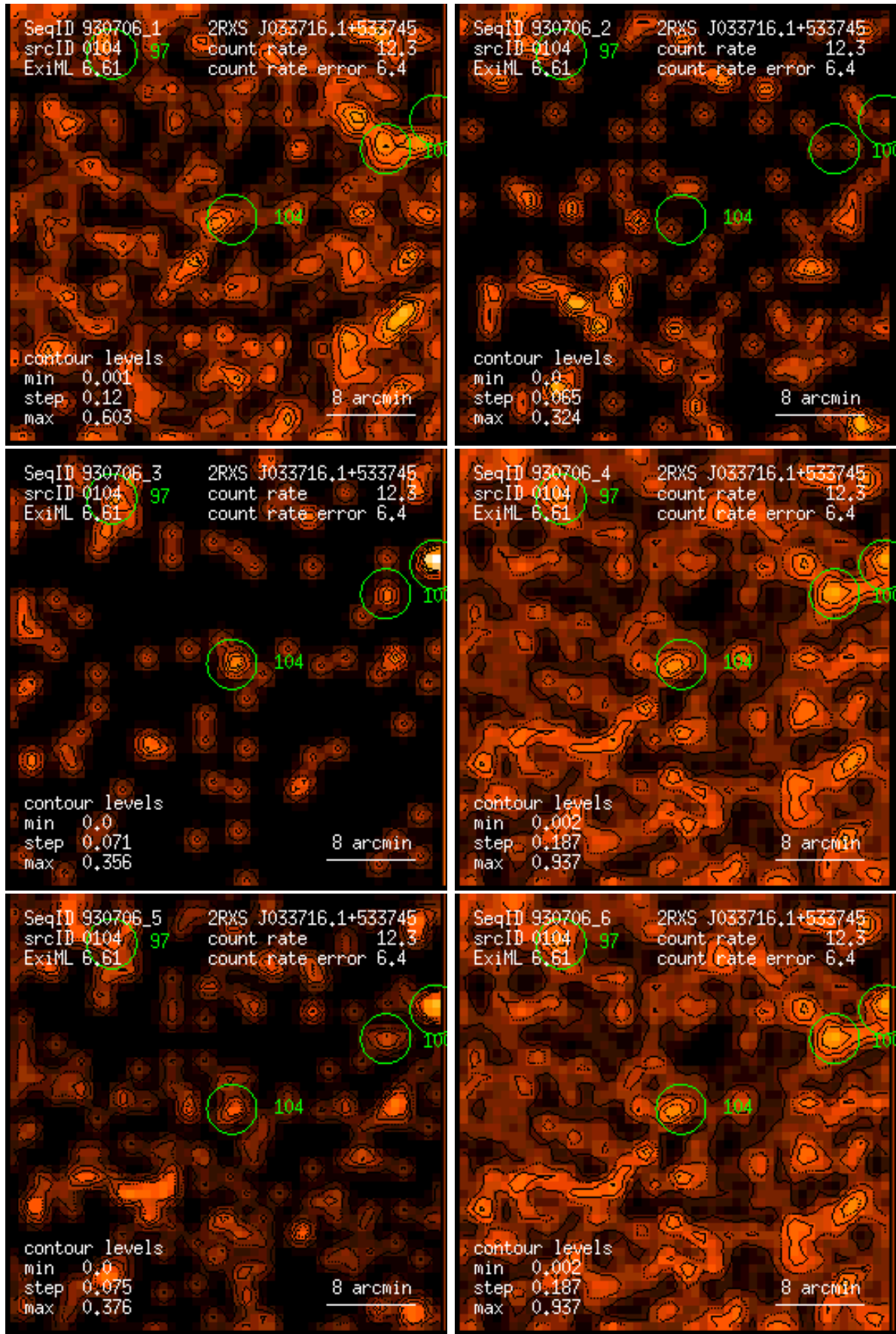
Figure 104: RASS 930706: detection 0104: band rate images, Gaussian filter: (1) PSPC channels 11 – 41, (2) 52 – 90, (3) 91 – 201, (4) 11 – 235, (5) 52 – 201, (6) 11 – 201. Broad band rates in counts/ks. Band rate contour levels in counts/ks/arcmin 2 .
