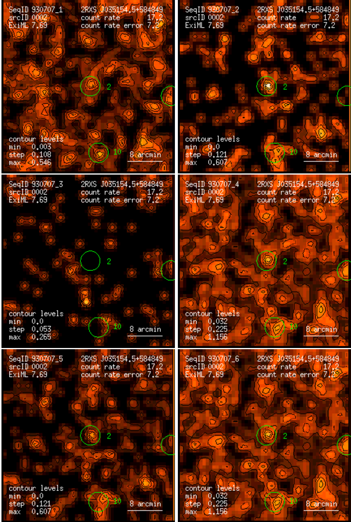
Figure 2: RASS 930707: detection 0002: band rate images, Gaussian filter: (1) PSPC channels 11 – 41, (2) 52 – 90, (3) 91 – 201, (4) 11 – 235, (5) 52 – 201, (6) 11 – 201. Broad band rates in counts/ks. Band rate contour levels in counts/ks/arcmin 2 .
