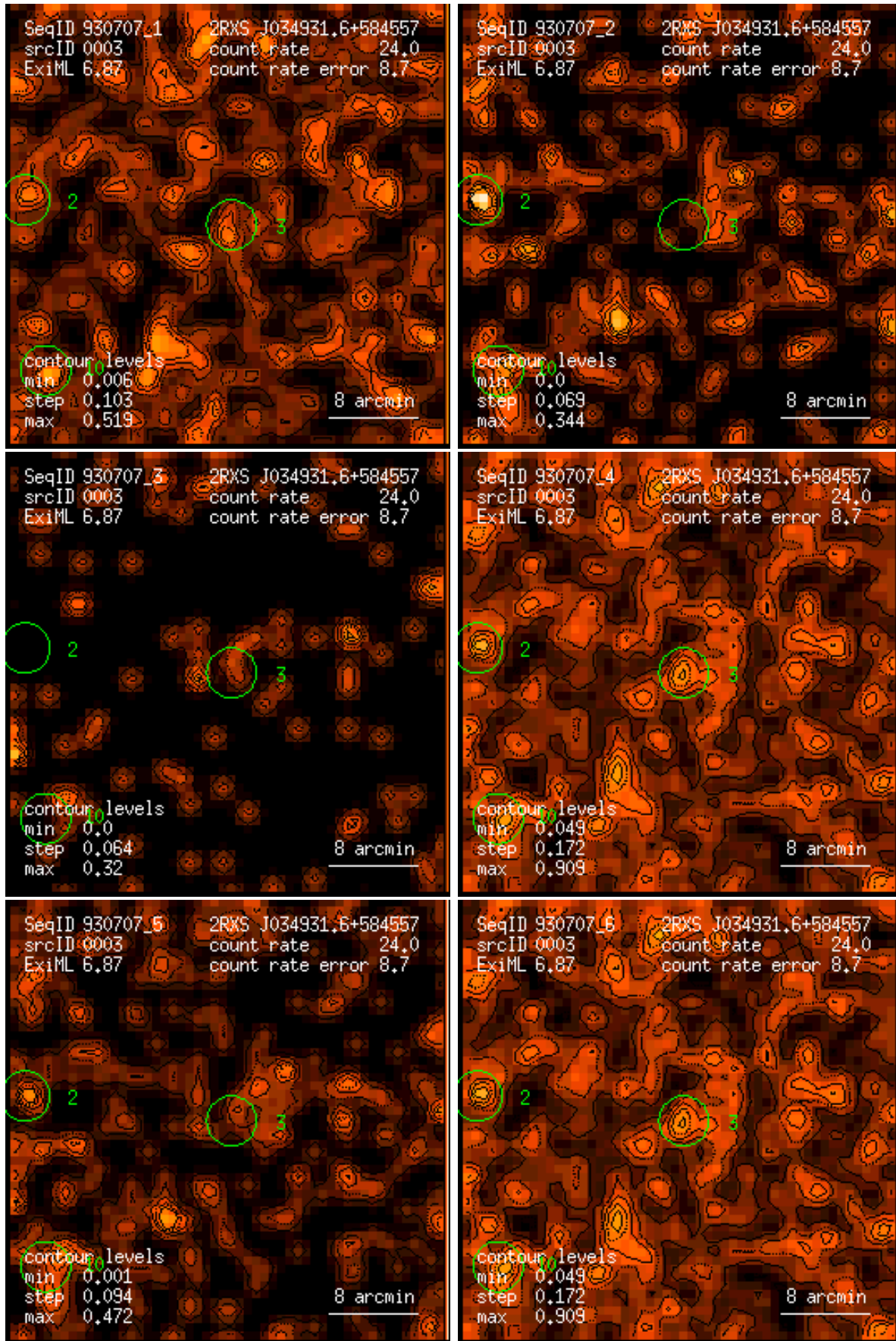
Figure 3: RASS 930707: detection 0003: band rate images, Gaussian filter: (1) PSPC channels 11 – 41, (2) 52 – 90, (3) 91 – 201, (4) 11 – 235, (5) 52 – 201, (6) 11 – 201. Broad band rates in counts/ks. Band rate contour levels in counts/ks/arcmin 2 .
