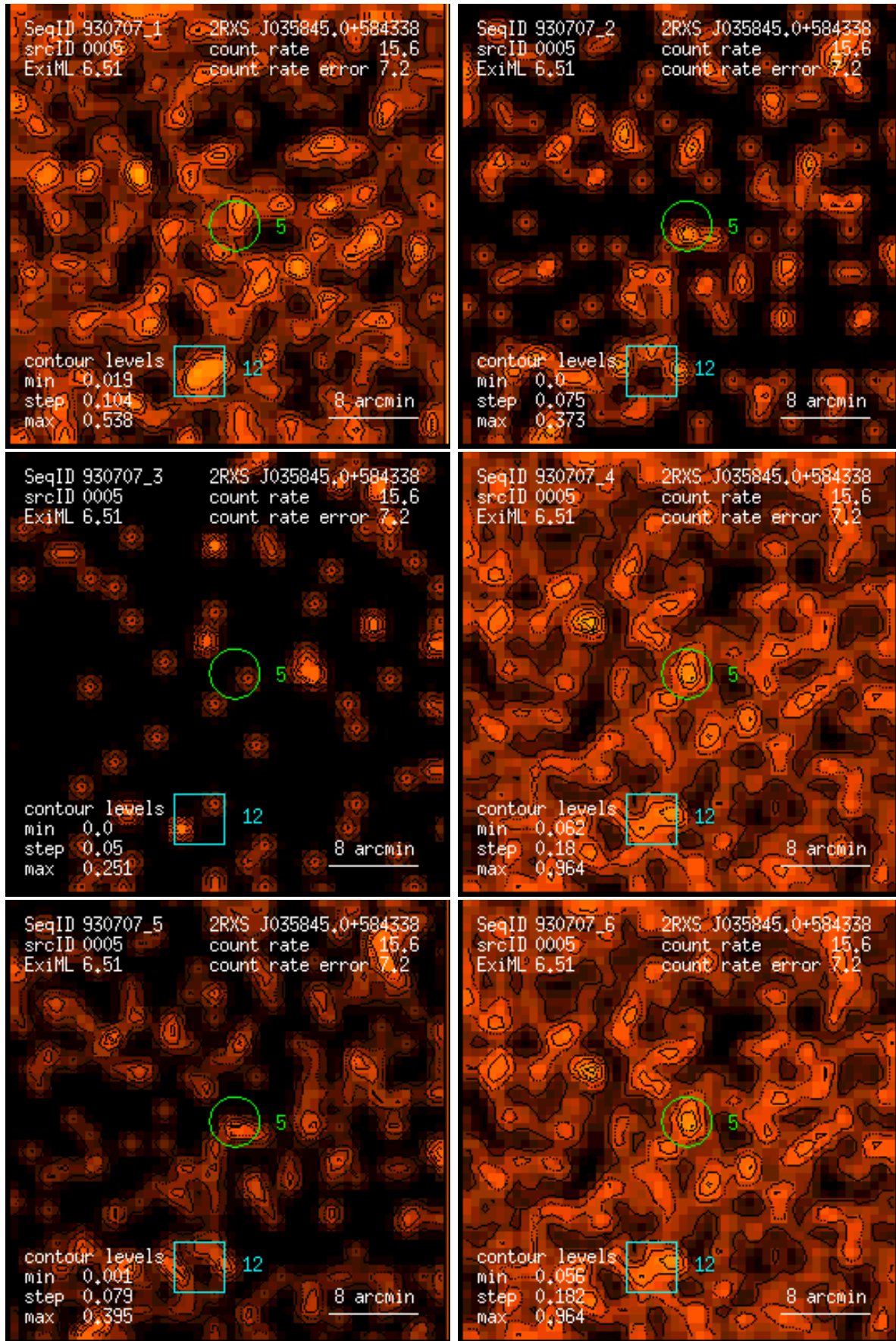
Figure 5: RASS 930707: detection 0005: band rate images, Gaussian filter: (1) PSPC channels 11 – 41, (2) 52 – 90, (3) 91 – 201, (4) 11 – 235, (5) 52 – 201, (6) 11 – 201. Broad band rates in counts/ks. Band rate contour levels in counts/ks/arcmin 2 .
