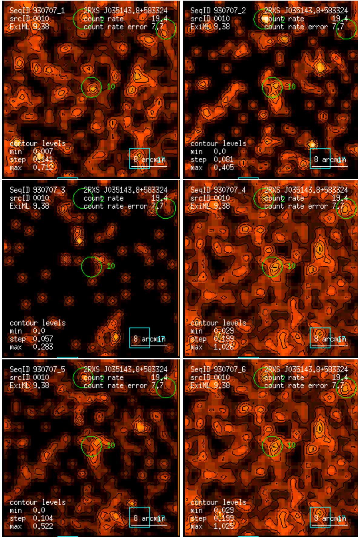
Figure 10: RASS 930707: detection 0010: band rate images, Gaussian filter: (1) PSPC channels 11 – 41, (2) 52 – 90, (3) 91 – 201, (4) 11 – 235, (5) 52 – 201, (6) 11 – 201. Broad band rates in counts/ks. Band rate contour levels in counts/ks/arcmin 2 .
