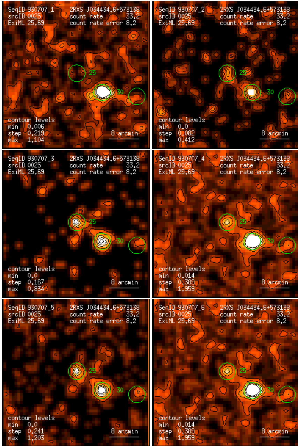
Figure 25: RASS 930707: detection 0025: band rate images, Gaussian filter: (1) PSPC channels 11 – 41, (2) 52 – 90, (3) 91 – 201, (4) 11 – 235, (5) 52 – 201, (6) 11 – 201. Broad band rates in counts/ks. Band rate contour levels in counts/ks/arcmin 2 .
