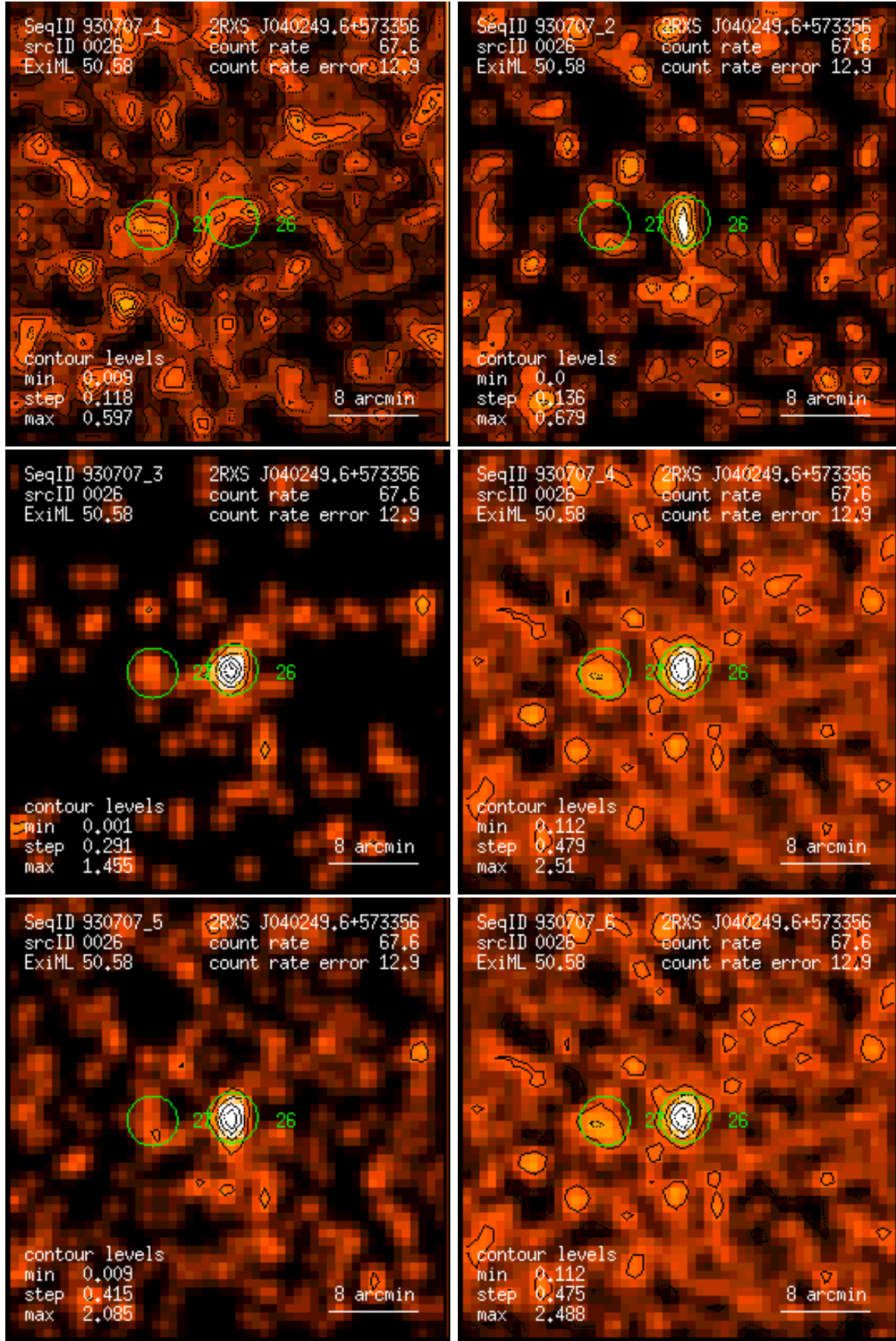
Figure 26: RASS 930707: detection 0026: band rate images, Gaussian filter: (1) PSPC channels 11 – 41, (2) 52 – 90, (3) 91 – 201, (4) 11 – 235, (5) 52 – 201, (6) 11 – 201. Broad band rates in counts/ks. Band rate contour levels in counts/ks/arcmin 2 .
