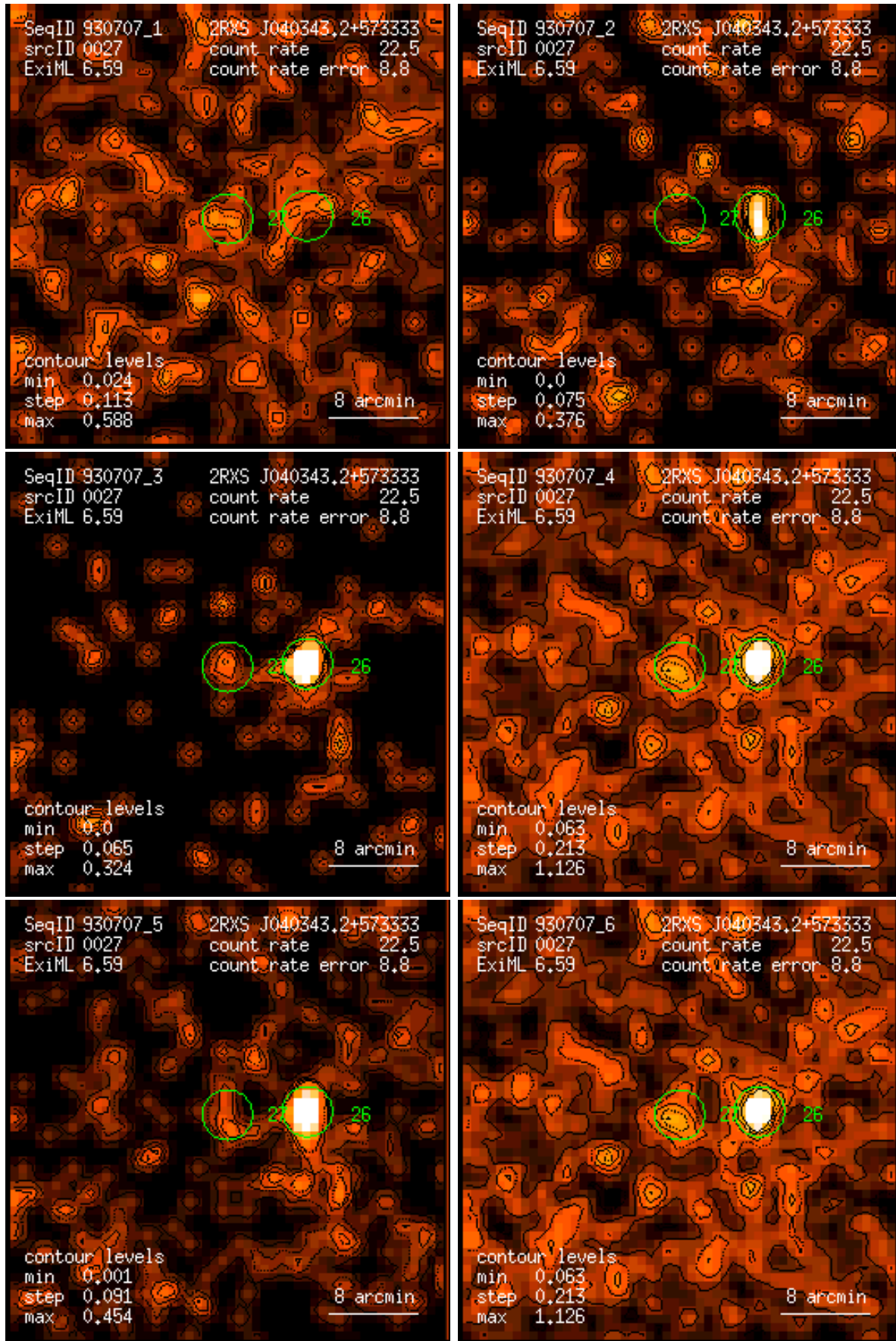
Figure 27: RASS 930707: detection 0027: band rate images, Gaussian filter: (1) PSPC channels 11 – 41, (2) 52 – 90, (3) 91 – 201, (4) 11 – 235, (5) 52 – 201, (6) 11 – 201. Broad band rates in counts/ks. Band rate contour levels in counts/ks/arcmin 2 .
