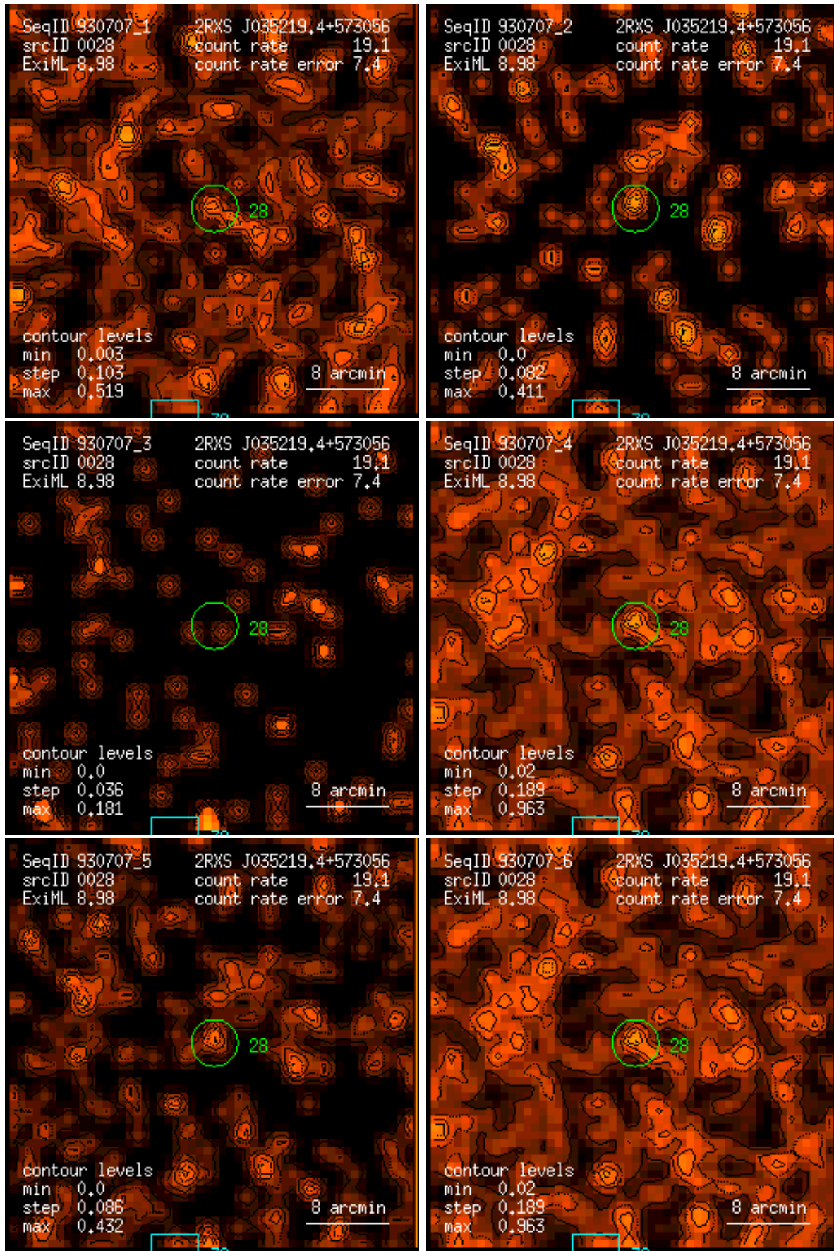
Figure 28: RASS 930707: detection 0028: band rate images, Gaussian filter: (1) PSPC channels 11 – 41, (2) 52 – 90, (3) 91 – 201, (4) 11 – 235, (5) 52 – 201, (6) 11 – 201. Broad band rates in counts/ks. Band rate contour levels in counts/ks/arcmin 2 .
