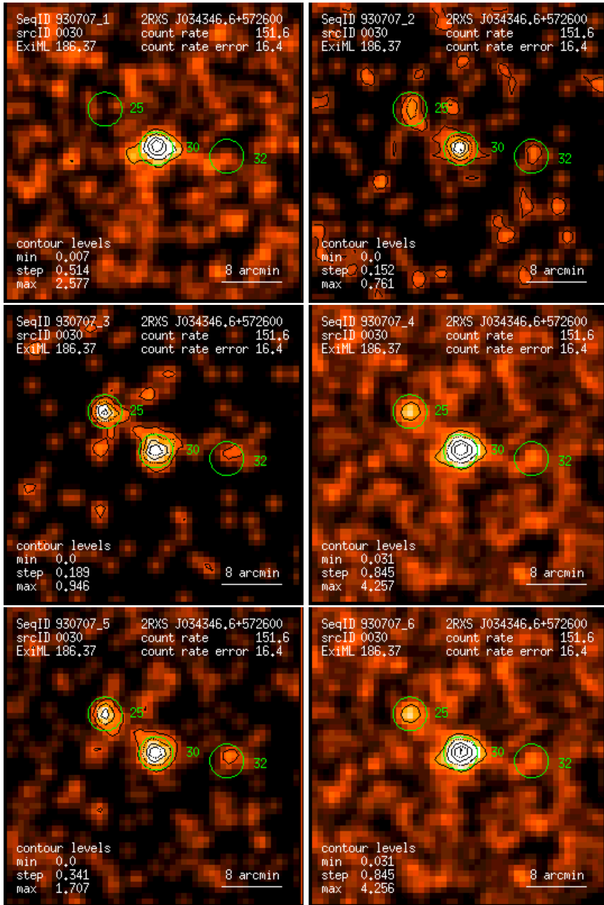
Figure 30: RASS 930707: detection 0030: band rate images, Gaussian filter: (1) PSPC channels 11 – 41, (2) 52 – 90, (3) 91 – 201, (4) 11 – 235, (5) 52 – 201, (6) 11 – 201. Broad band rates in counts/ks. Band rate contour levels in counts/ks/arcmin 2 .
