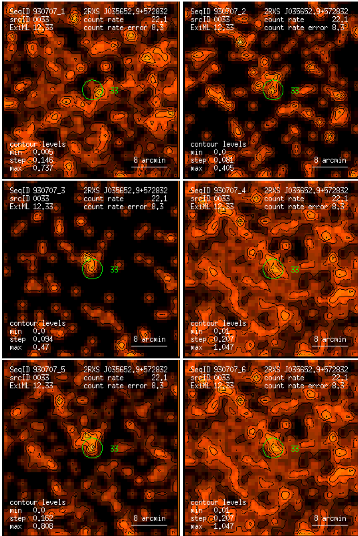
Figure 33: RASS 930707: detection 0033: band rate images, Gaussian filter: (1) PSPC channels 11 – 41, (2) 52 – 90, (3) 91 – 201, (4) 11 – 235, (5) 52 – 201, (6) 11 – 201. Broad band rates in counts/ks. Band rate contour levels in counts/ks/arcmin 2 .
