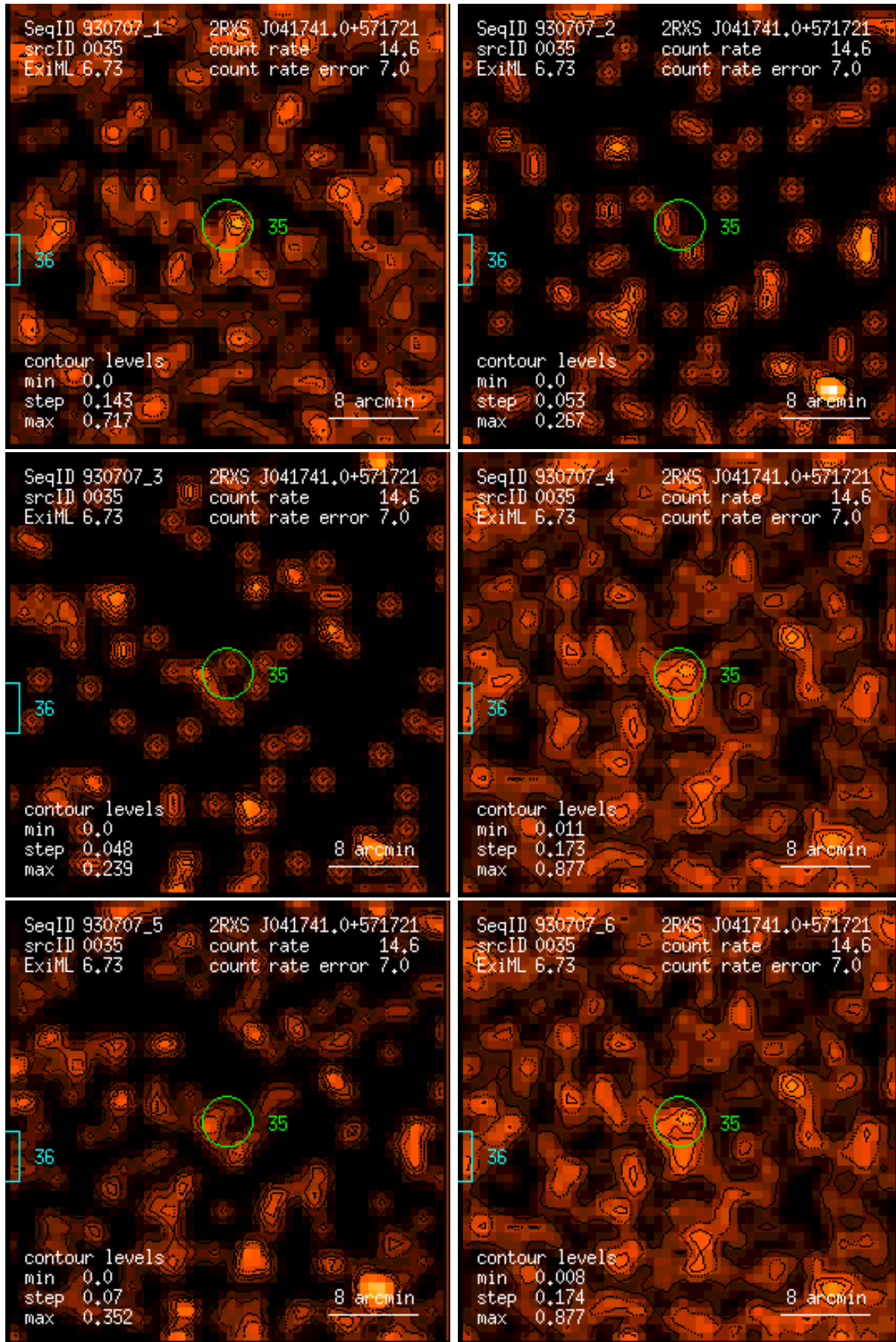
Figure 35: RASS 930707: detection 0035: band rate images, Gaussian filter: (1) PSPC channels 11 – 41, (2) 52 – 90, (3) 91 – 201, (4) 11 – 235, (5) 52 – 201, (6) 11 – 201. Broad band rates in counts/ks. Band rate contour levels in counts/ks/arcmin 2 .
