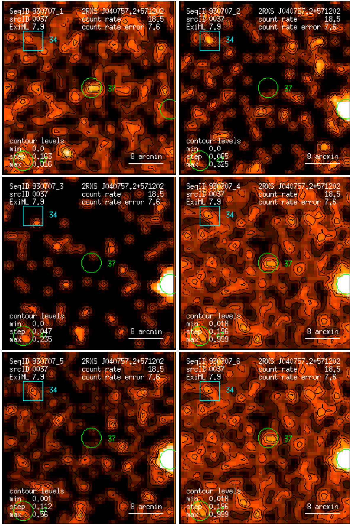
Figure 37: RASS 930707: detection 0037: band rate images, Gaussian filter: (1) PSPC channels 11 – 41, (2) 52 – 90, (3) 91 – 201, (4) 11 – 235, (5) 52 – 201, (6) 11 – 201. Broad band rates in counts/ks. Band rate contour levels in counts/ks/arcmin 2 .
