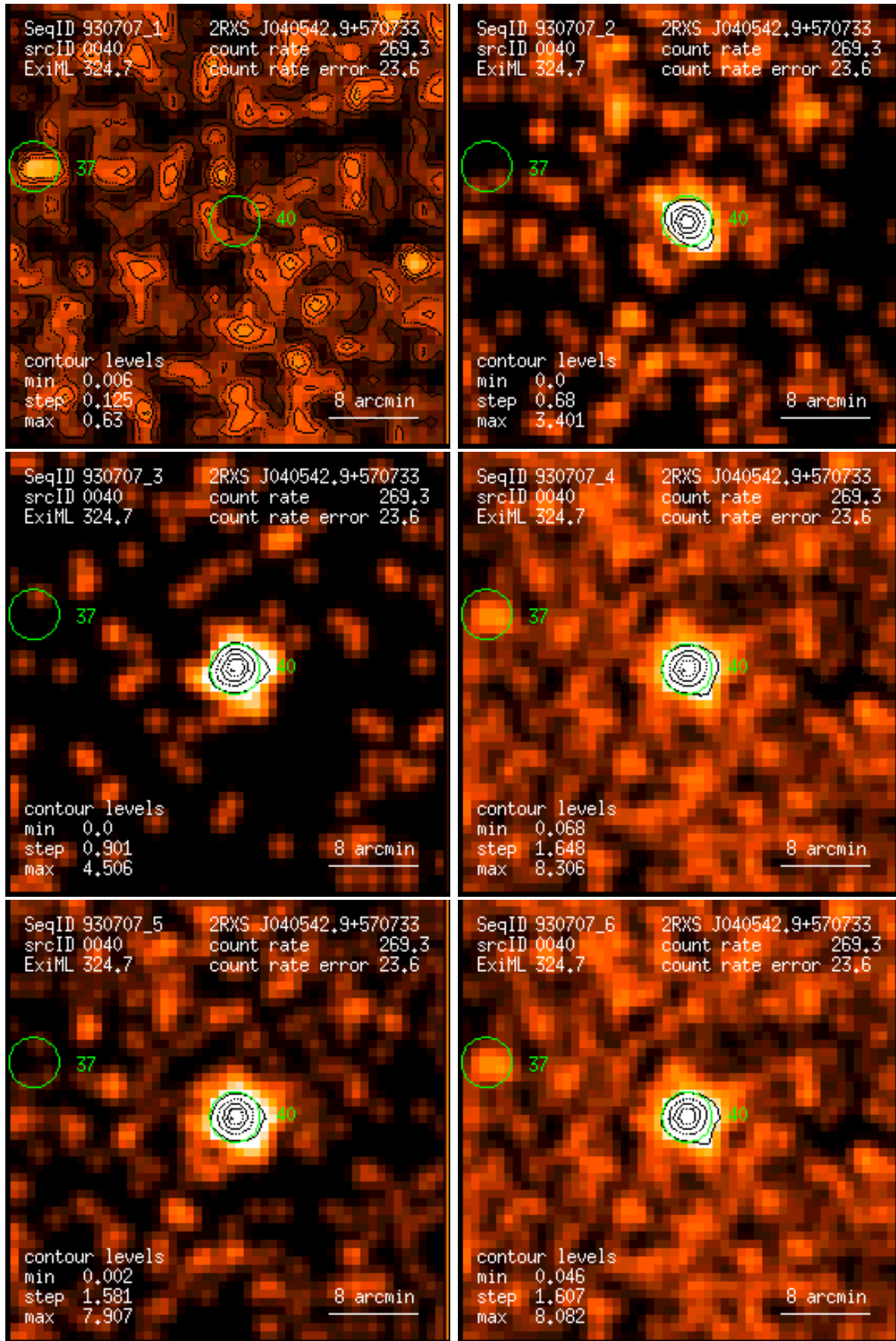
Figure 40: RASS 930707: detection 0040: band rate images, Gaussian filter: (1) PSPC channels 11 – 41, (2) 52 – 90, (3) 91 – 201, (4) 11 – 235, (5) 52 – 201, (6) 11 – 201. Broad band rates in counts/ks. Band rate contour levels in counts/ks/arcmin 2 .
