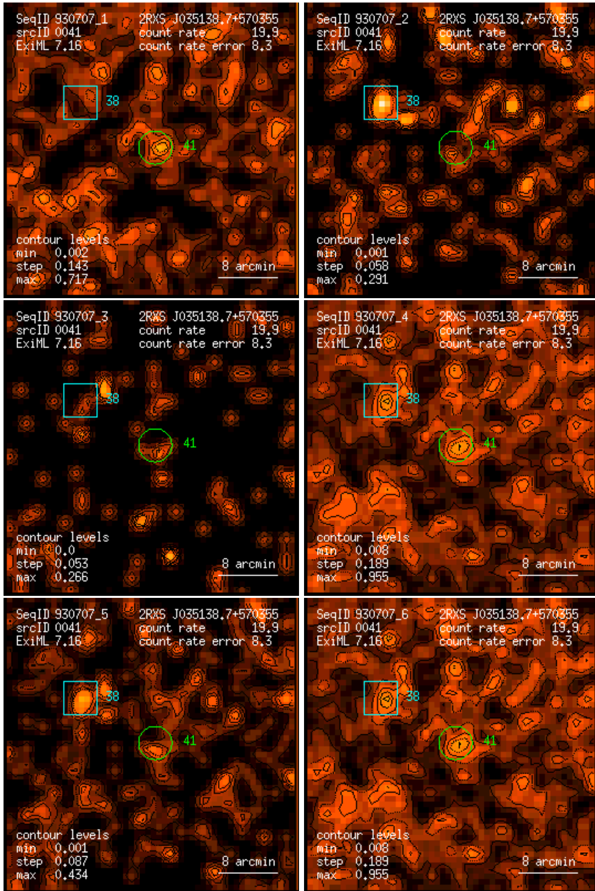
Figure 41: RASS 930707: detection 0041: band rate images, Gaussian filter: (1) PSPC channels 11 – 41, (2) 52 – 90, (3) 91 – 201, (4) 11 – 235, (5) 52 – 201, (6) 11 – 201. Broad band rates in counts/ks. Band rate contour levels in counts/ks/arcmin 2 .
