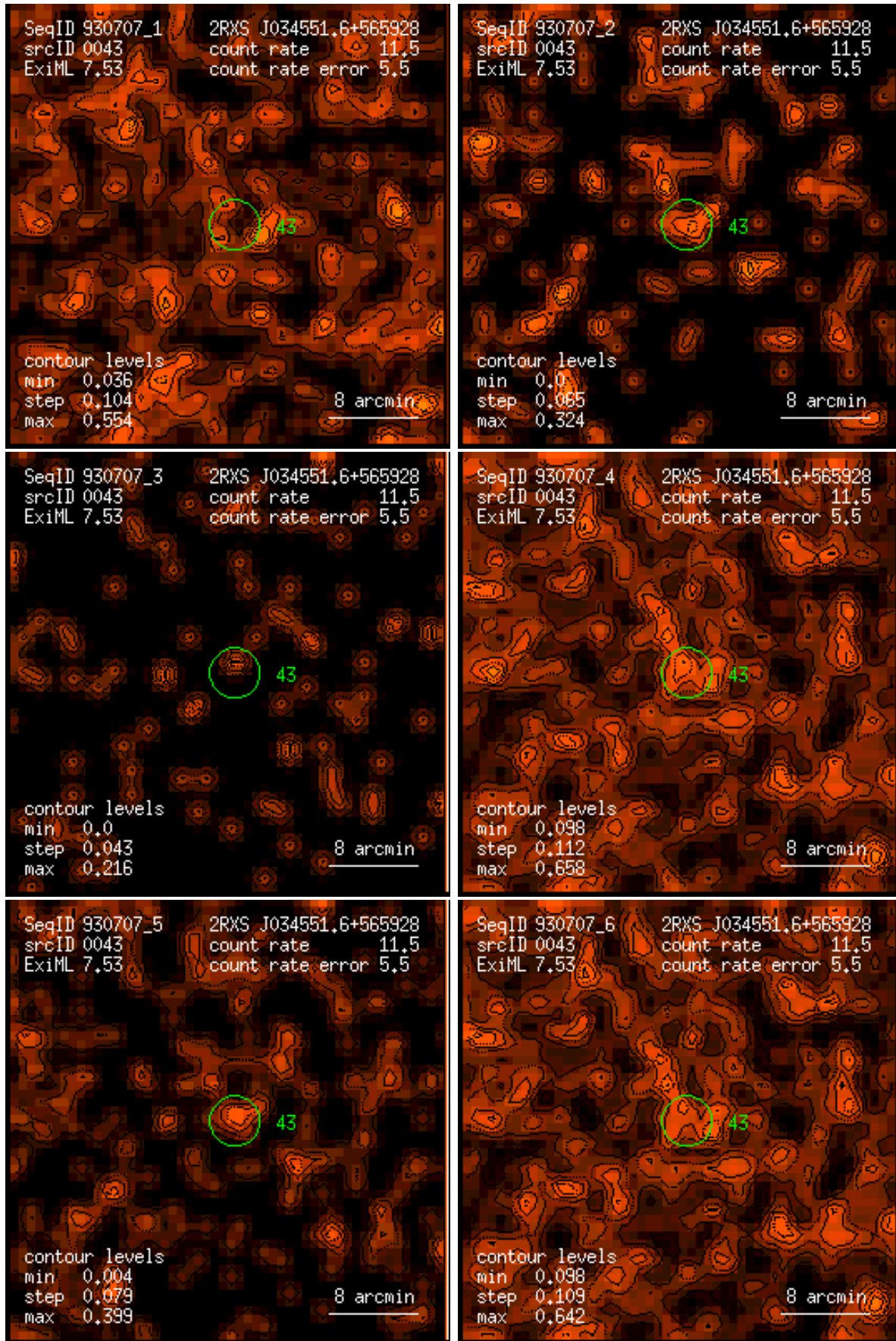
Figure 43: RASS 930707: detection 0043: band rate images, Gaussian filter: (1) PSPC channels 11 – 41, (2) 52 – 90, (3) 91 – 201, (4) 11 – 235, (5) 52 – 201, (6) 11 – 201. Broad band rates in counts/ks. Band rate contour levels in counts/ks/arcmin 2 .
