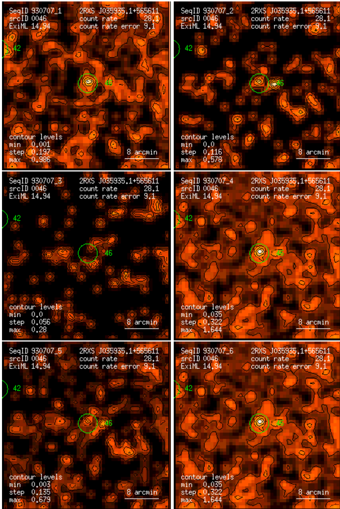
Figure 46: RASS 930707: detection 0046: band rate images, Gaussian filter: (1) PSPC channels 11 – 41, (2) 52 – 90, (3) 91 – 201, (4) 11 – 235, (5) 52 – 201, (6) 11 – 201. Broad band rates in counts/ks. Band rate contour levels in counts/ks/arcmin 2 .
