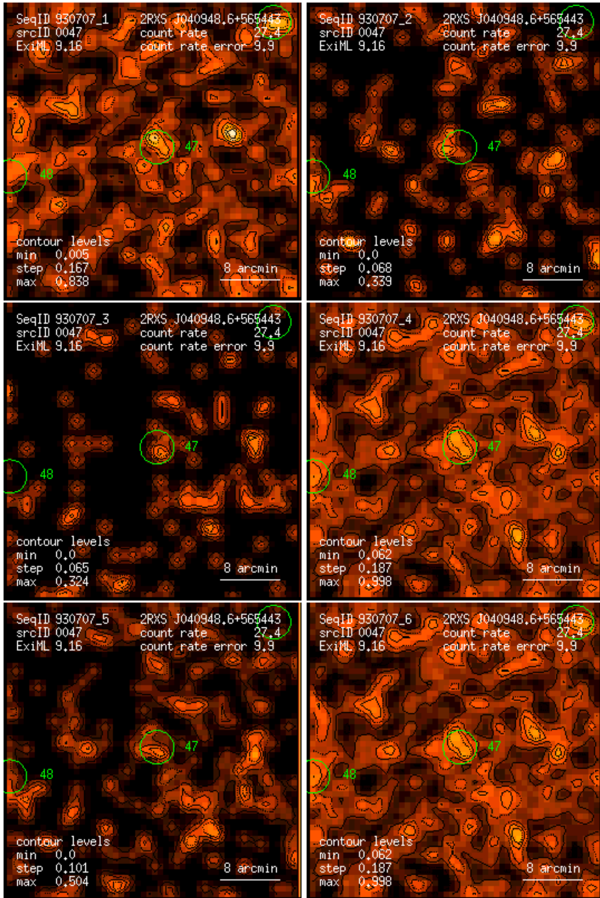
Figure 47: RASS 930707: detection 0047: band rate images, Gaussian filter: (1) PSPC channels 11 – 41, (2) 52 – 90, (3) 91 – 201, (4) 11 – 235, (5) 52 – 201, (6) 11 – 201. Broad band rates in counts/ks. Band rate contour levels in counts/ks/arcmin 2 .
