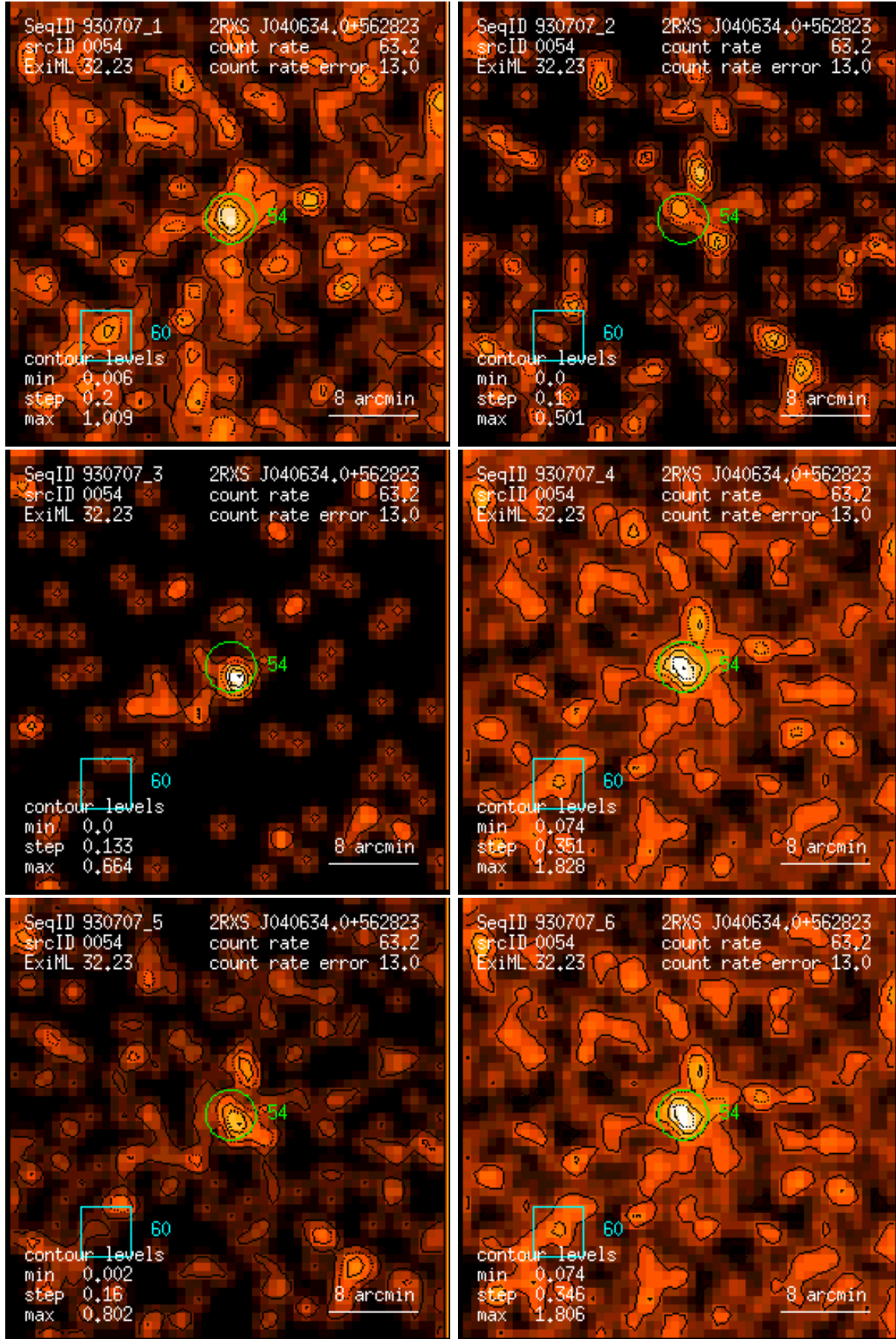
Figure 54: RASS 930707: detection 0054: band rate images, Gaussian filter: (1) PSPC channels 11 – 41, (2) 52 – 90, (3) 91 – 201, (4) 11 – 235, (5) 52 – 201, (6) 11 – 201. Broad band rates in counts/ks. Band rate contour levels in counts/ks/arcmin 2 .
