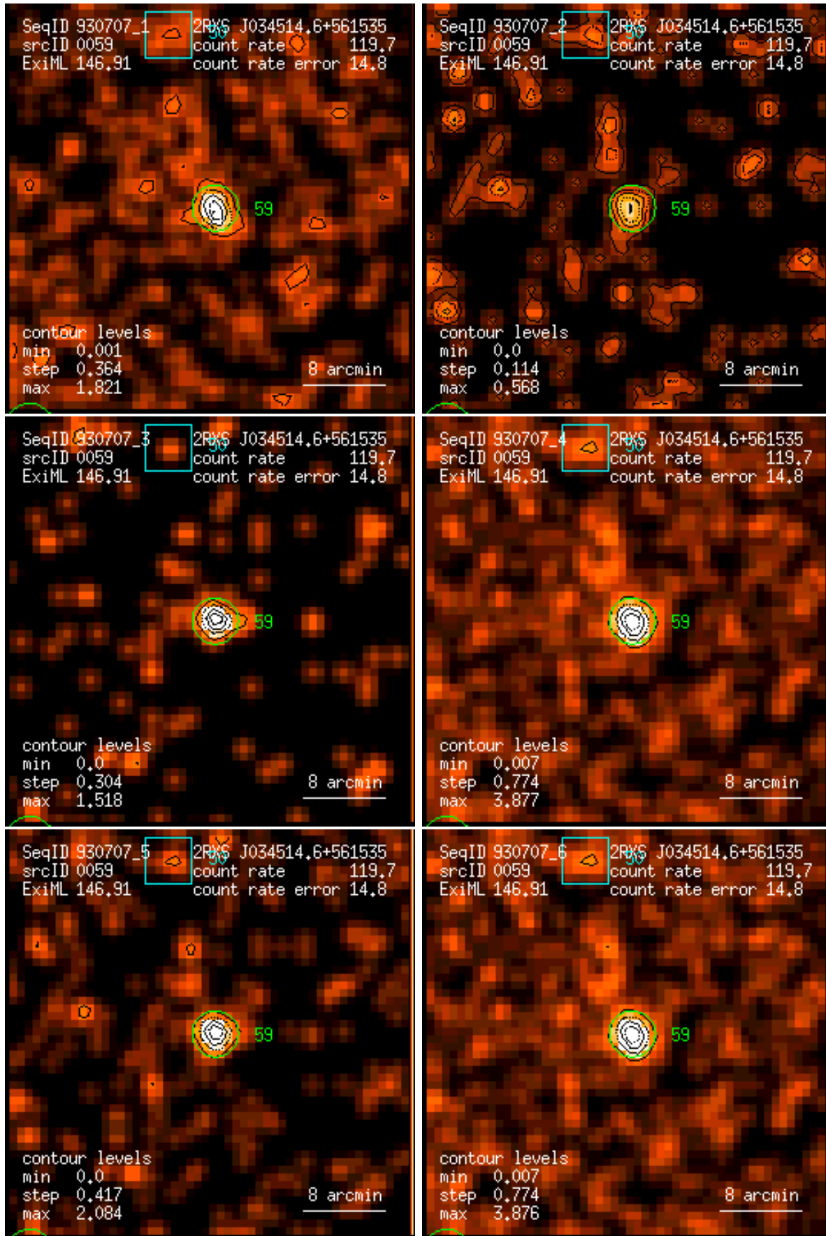
Figure 59: RASS 930707: detection 0059: band rate images, Gaussian filter: (1) PSPC channels 11 – 41, (2) 52 – 90, (3) 91 – 201, (4) 11 – 235, (5) 52 – 201, (6) 11 – 201. Broad band rates in counts/ks. Band rate contour levels in counts/ks/arcmin 2 .
