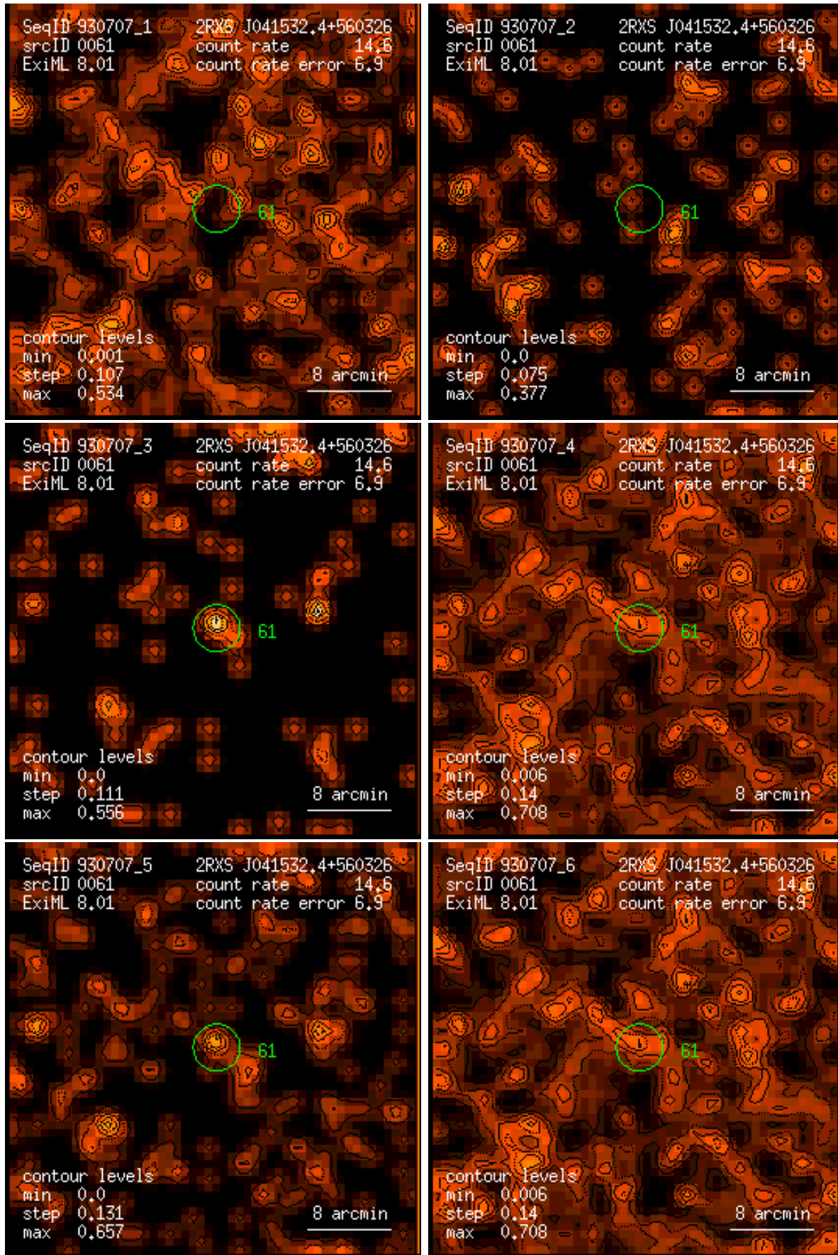
Figure 61: RASS 930707: detection 0061: band rate images, Gaussian filter: (1) PSPC channels 11 – 41, (2) 52 – 90, (3) 91 – 201, (4) 11 – 235, (5) 52 – 201, (6) 11 – 201. Broad band rates in counts/ks. Band rate contour levels in counts/ks/arcmin 2 .
