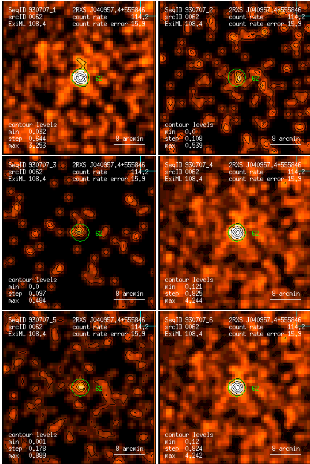
Figure 62: RASS 930707: detection 0062: band rate images, Gaussian filter: (1) PSPC channels 11 – 41, (2) 52 – 90, (3) 91 – 201, (4) 11 – 235, (5) 52 – 201, (6) 11 – 201. Broad band rates in counts/ks. Band rate contour levels in counts/ks/arcmin 2 .
