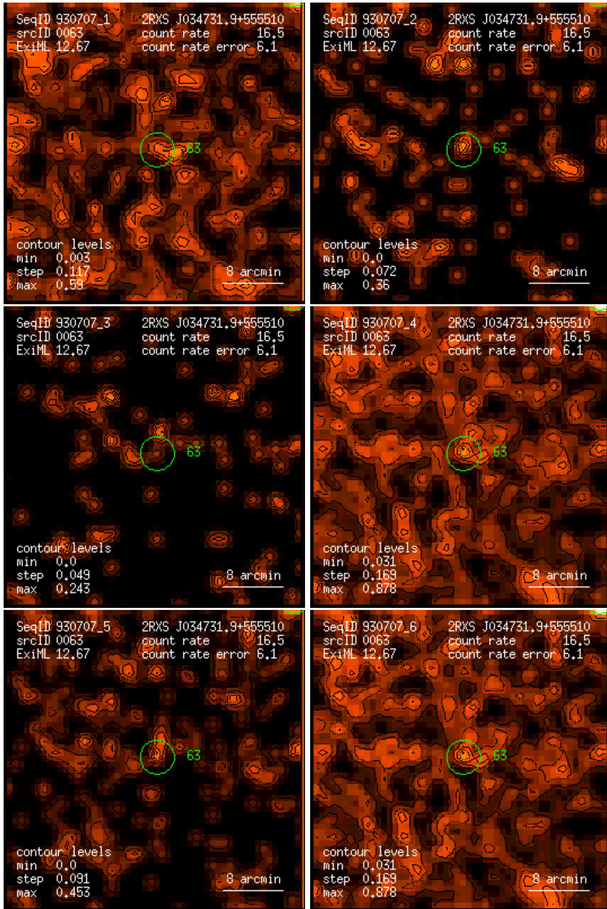
Figure 63: RASS 930707: detection 0063: band rate images, Gaussian filter: (1) PSPC channels 11 – 41, (2) 52 – 90, (3) 91 – 201, (4) 11 – 235, (5) 52 – 201, (6) 11 – 201. Broad band rates in counts/ks. Band rate contour levels in counts/ks/arcmin 2 .
