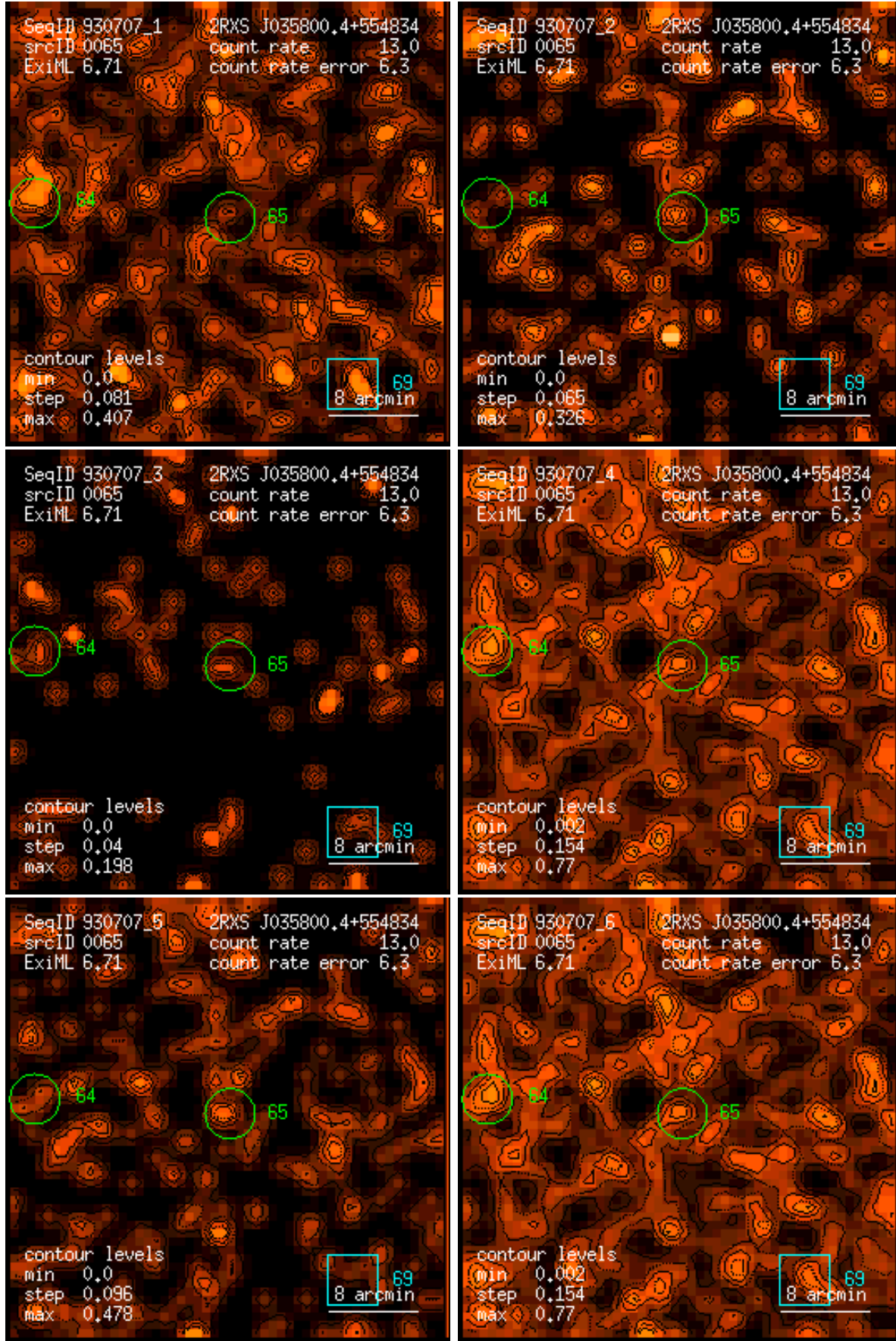
Figure 65: RASS 930707: detection 0065: band rate images, Gaussian filter: (1) PSPC channels 11 – 41, (2) 52 – 90, (3) 91 – 201, (4) 11 – 235, (5) 52 – 201, (6) 11 – 201. Broad band rates in counts/ks. Band rate contour levels in counts/ks/arcmin 2 .
