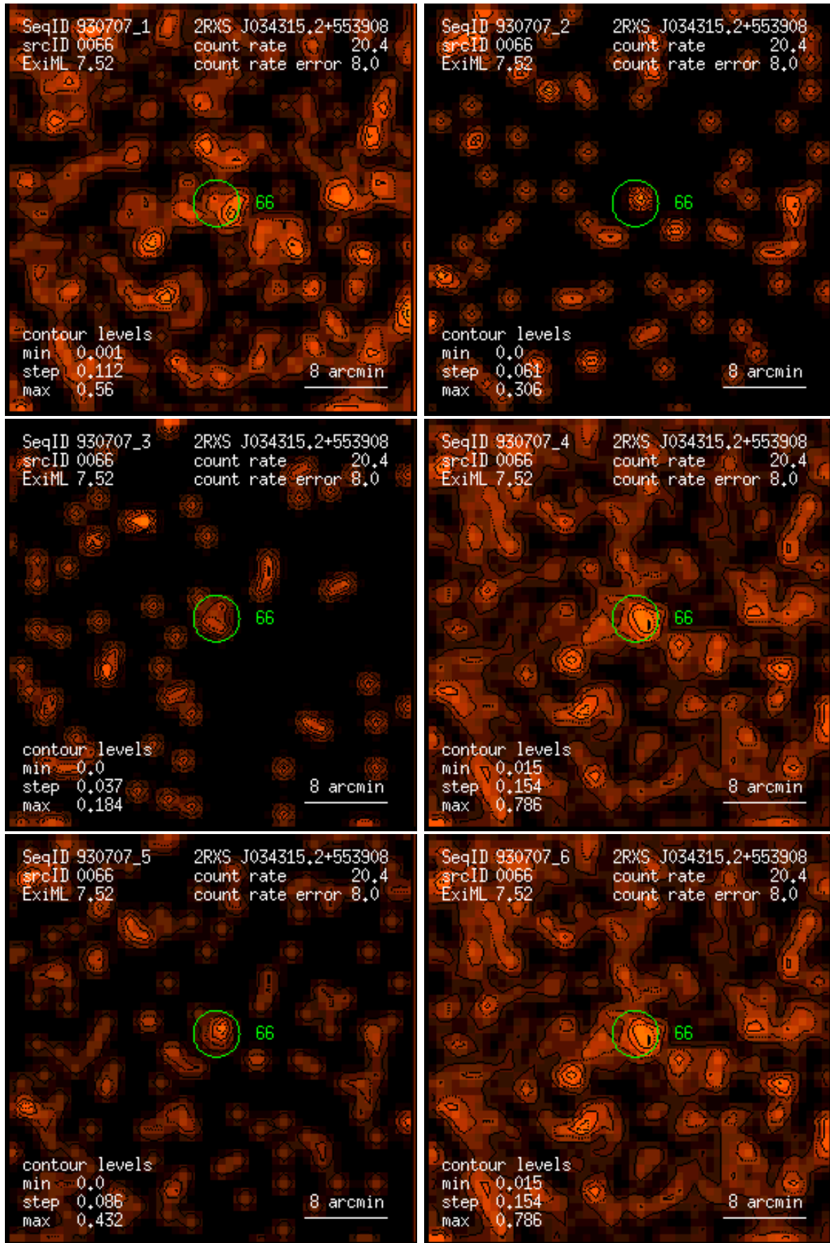
Figure 66: RASS 930707: detection 0066: band rate images, Gaussian filter: (1) PSPC channels 11 – 41, (2) 52 – 90, (3) 91 – 201, (4) 11 – 235, (5) 52 – 201, (6) 11 – 201. Broad band rates in counts/ks. Band rate contour levels in counts/ks/arcmin 2 .
