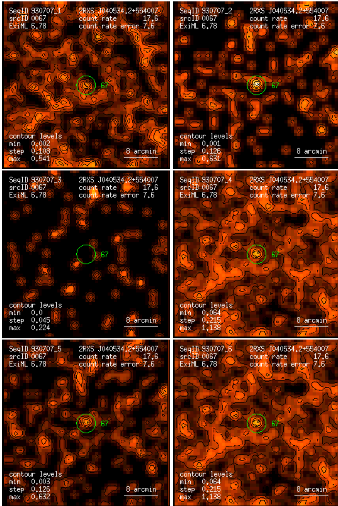
Figure 67: RASS 930707: detection 0067: band rate images, Gaussian filter: (1) PSPC channels 11 – 41, (2) 52 – 90, (3) 91 – 201, (4) 11 – 235, (5) 52 – 201, (6) 11 – 201. Broad band rates in counts/ks. Band rate contour levels in counts/ks/arcmin 2 .
