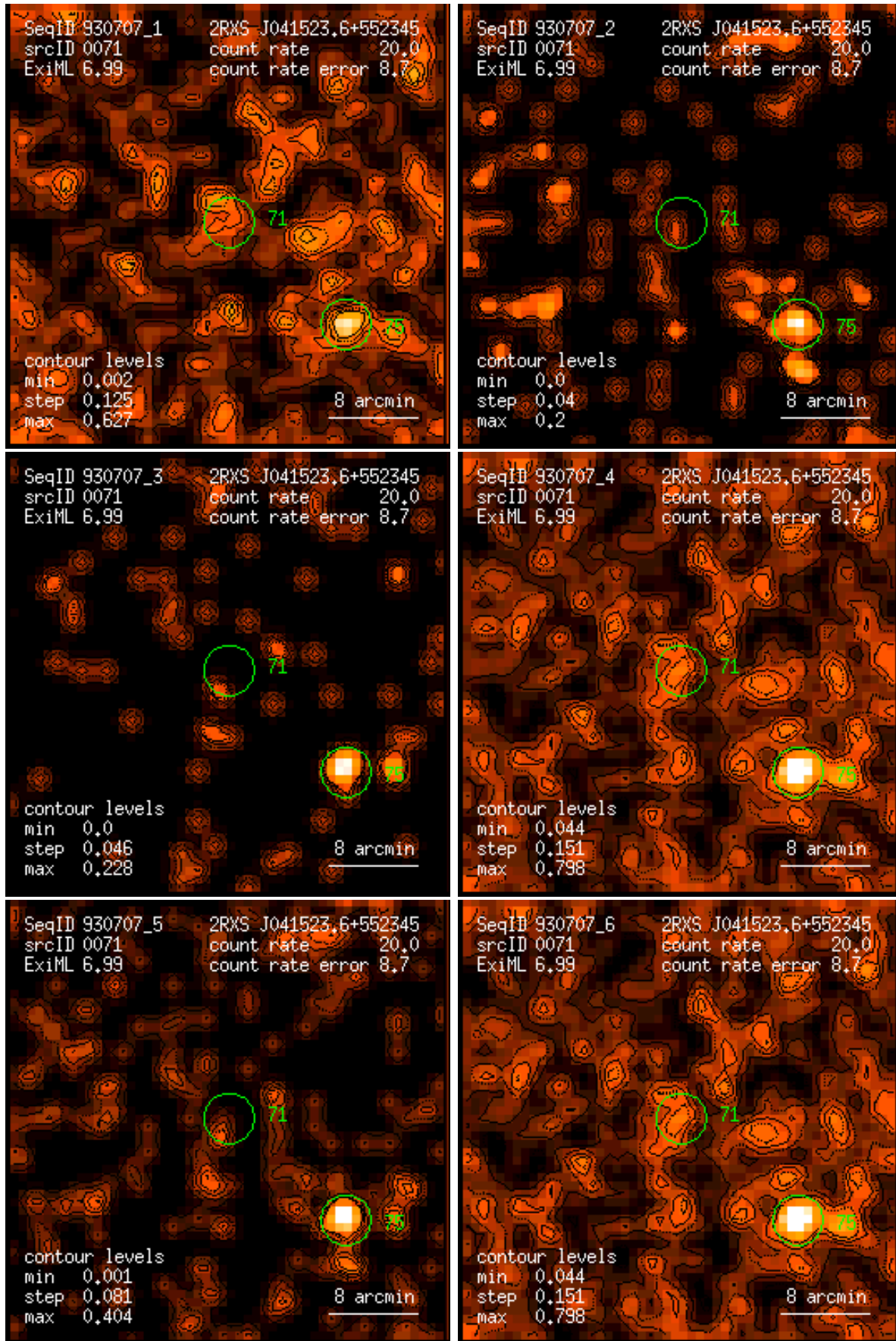
Figure 71: RASS 930707: detection 0071: band rate images, Gaussian filter: (1) PSPC channels 11 – 41, (2) 52 – 90, (3) 91 – 201, (4) 11 – 235, (5) 52 – 201, (6) 11 – 201. Broad band rates in counts/ks. Band rate contour levels in counts/ks/arcmin 2 .
