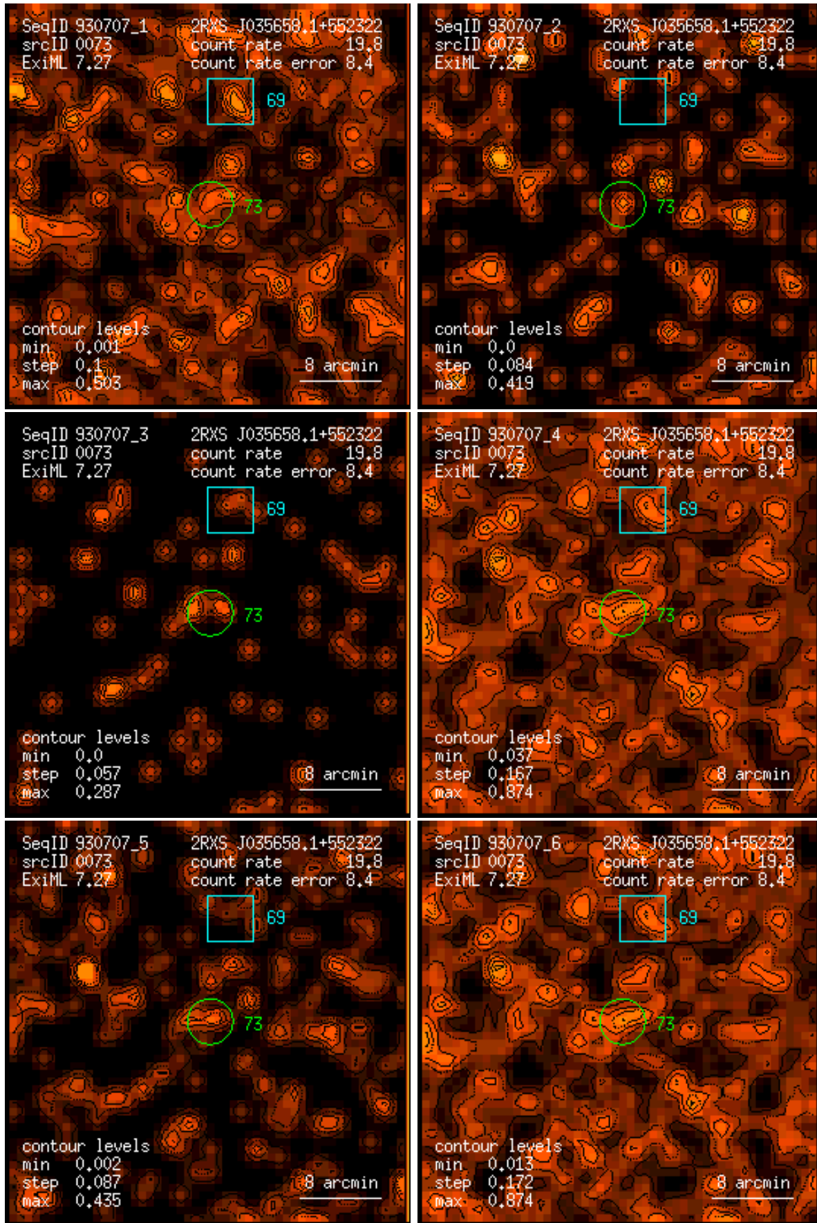
Figure 73: RASS 930707: detection 0073: band rate images, Gaussian filter: (1) PSPC channels 11 – 41, (2) 52 – 90, (3) 91 – 201, (4) 11 – 235, (5) 52 – 201, (6) 11 – 201. Broad band rates in counts/ks. Band rate contour levels in counts/ks/arcmin 2 .
