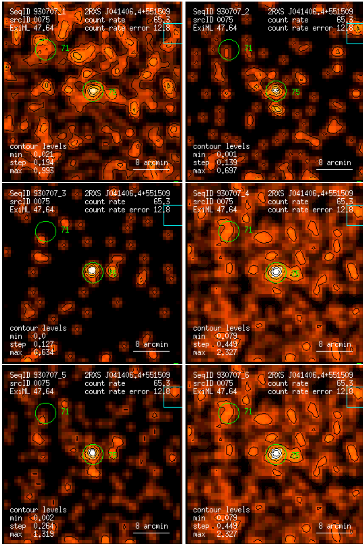
Figure 75: RASS 930707: detection 0075: band rate images, Gaussian filter: (1) PSPC channels 11 – 41, (2) 52 – 90, (3) 91 – 201, (4) 11 – 235, (5) 52 – 201, (6) 11 – 201. Broad band rates in counts/ks. Band rate contour levels in counts/ks/arcmin 2 .
