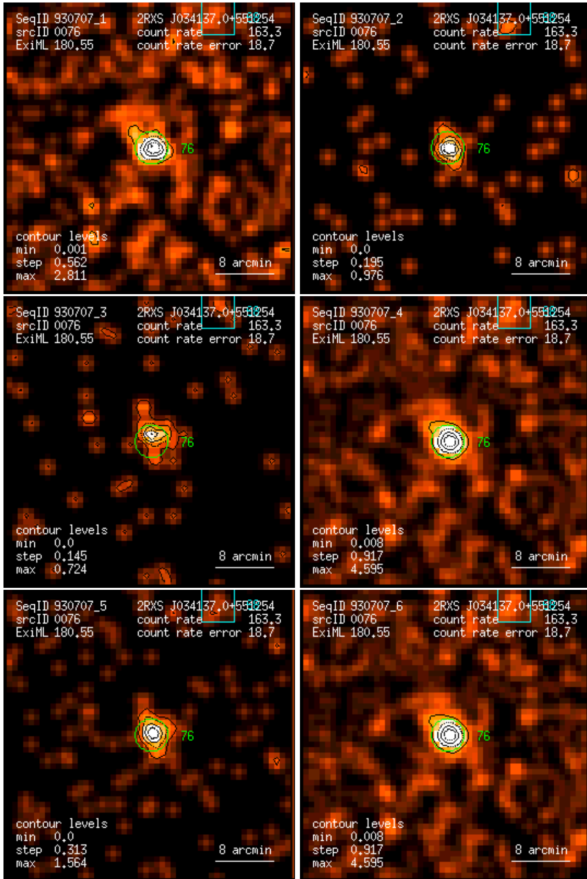
Figure 76: RASS 930707: detection 0076: band rate images, Gaussian filter: (1) PSPC channels 11 – 41, (2) 52 – 90, (3) 91 – 201, (4) 11 – 235, (5) 52 – 201, (6) 11 – 201. Broad band rates in counts/ks. Band rate contour levels in counts/ks/arcmin 2 .
