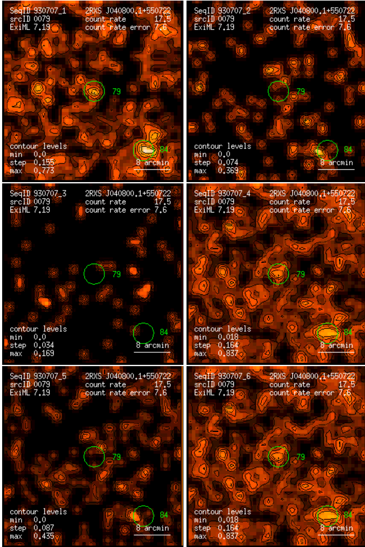
Figure 79: RASS 930707: detection 0079: band rate images, Gaussian filter: (1) PSPC channels 11 – 41, (2) 52 – 90, (3) 91 – 201, (4) 11 – 235, (5) 52 – 201, (6) 11 – 201. Broad band rates in counts/ks. Band rate contour levels in counts/ks/arcmin 2 .
