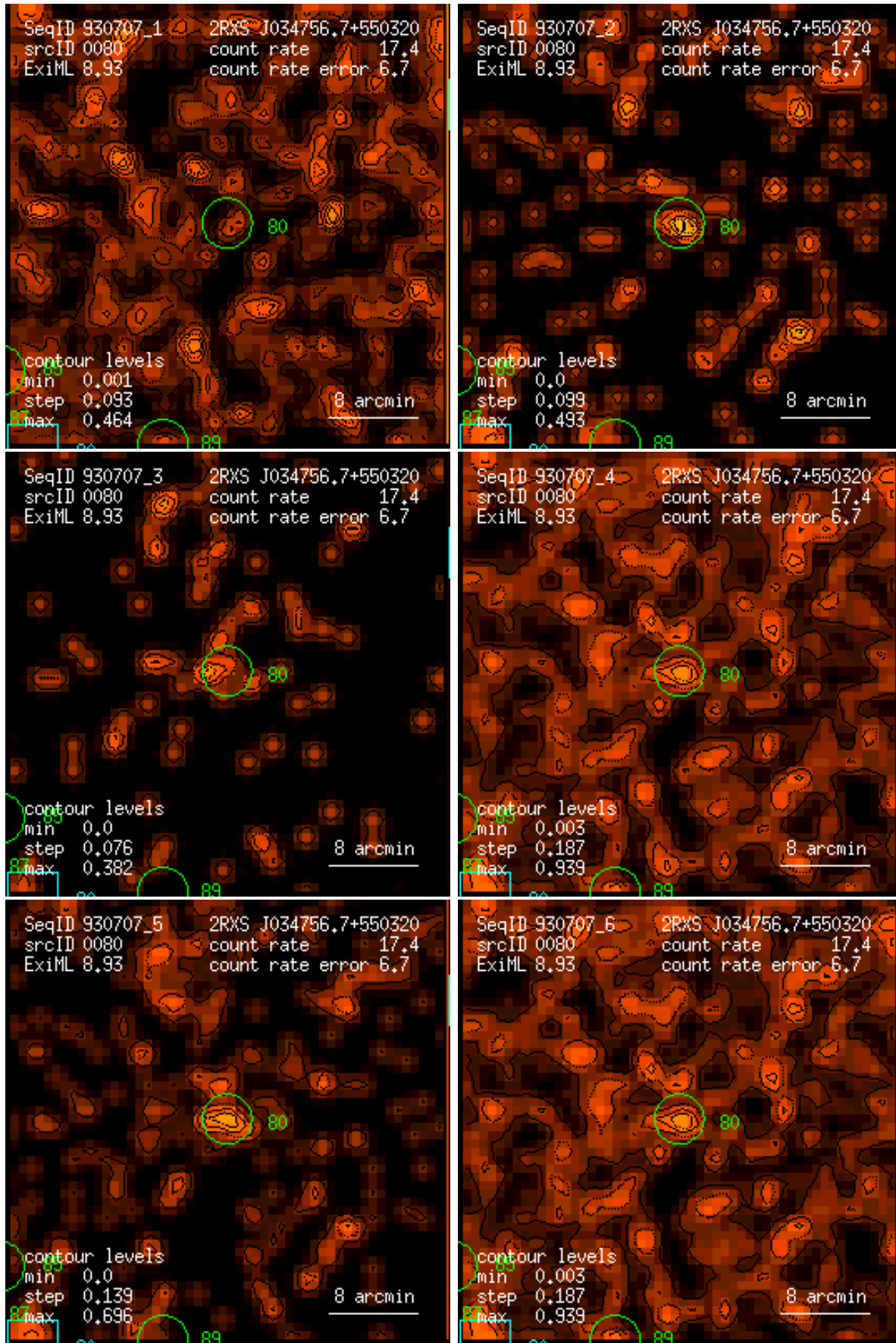
Figure 80: RASS 930707: detection 0080: band rate images, Gaussian filter: (1) PSPC channels 11 – 41, (2) 52 – 90, (3) 91 – 201, (4) 11 – 235, (5) 52 – 201, (6) 11 – 201. Broad band rates in counts/ks. Band rate contour levels in counts/ks/arcmin 2 .
