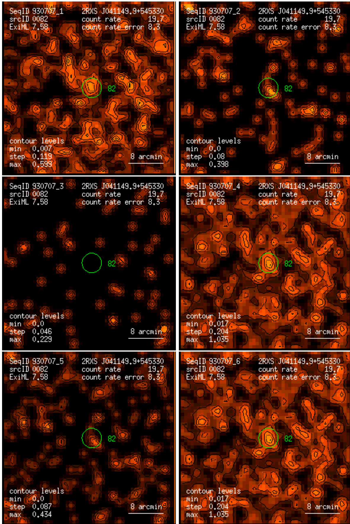
Figure 82: RASS 930707: detection 0082: band rate images, Gaussian filter: (1) PSPC channels 11 – 41, (2) 52 – 90, (3) 91 – 201, (4) 11 – 235, (5) 52 – 201, (6) 11 – 201. Broad band rates in counts/ks. Band rate contour levels in counts/ks/arcmin 2 .
