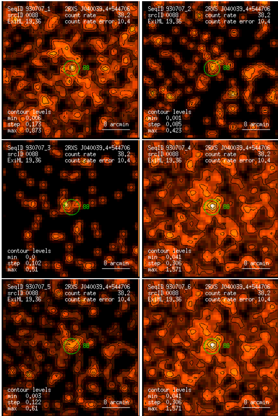
Figure 88: RASS 930707: detection 0088: band rate images, Gaussian filter: (1) PSPC channels 11 – 41, (2) 52 – 90, (3) 91 – 201, (4) 11 – 235, (5) 52 – 201, (6) 11 – 201. Broad band rates in counts/ks. Band rate contour levels in counts/ks/arcmin 2 .
