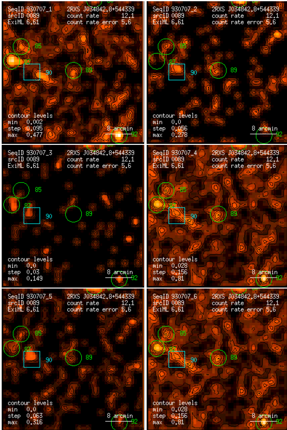
Figure 89: RASS 930707: detection 0089: band rate images, Gaussian filter: (1) PSPC channels 11 – 41, (2) 52 – 90, (3) 91 – 201, (4) 11 – 235, (5) 52 – 201, (6) 11 – 201. Broad band rates in counts/ks. Band rate contour levels in counts/ks/arcmin 2 .
