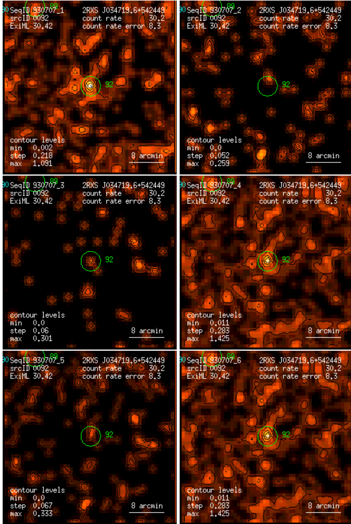
Figure 92: RASS 930707: detection 0092: band rate images, Gaussian filter: (1) PSPC channels 11 – 41, (2) 52 – 90, (3) 91 – 201, (4) 11 – 235, (5) 52 – 201, (6) 11 – 201. Broad band rates in counts/ks. Band rate contour levels in counts/ks/arcmin 2 .
