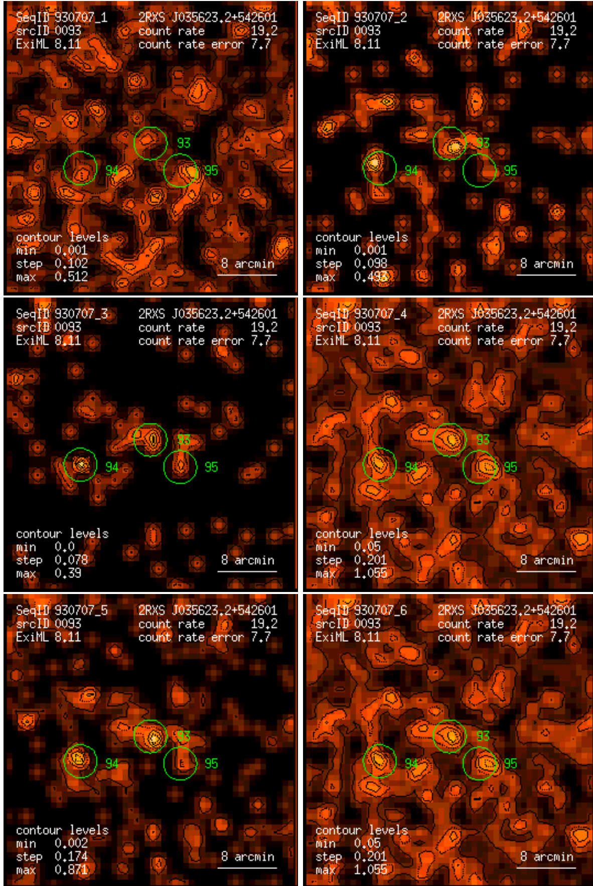
Figure 93: RASS 930707: detection 0093: band rate images, Gaussian filter: (1) PSPC channels 11 – 41, (2) 52 – 90, (3) 91 – 201, (4) 11 – 235, (5) 52 – 201, (6) 11 – 201. Broad band rates in counts/ks. Band rate contour levels in counts/ks/arcmin 2 .
