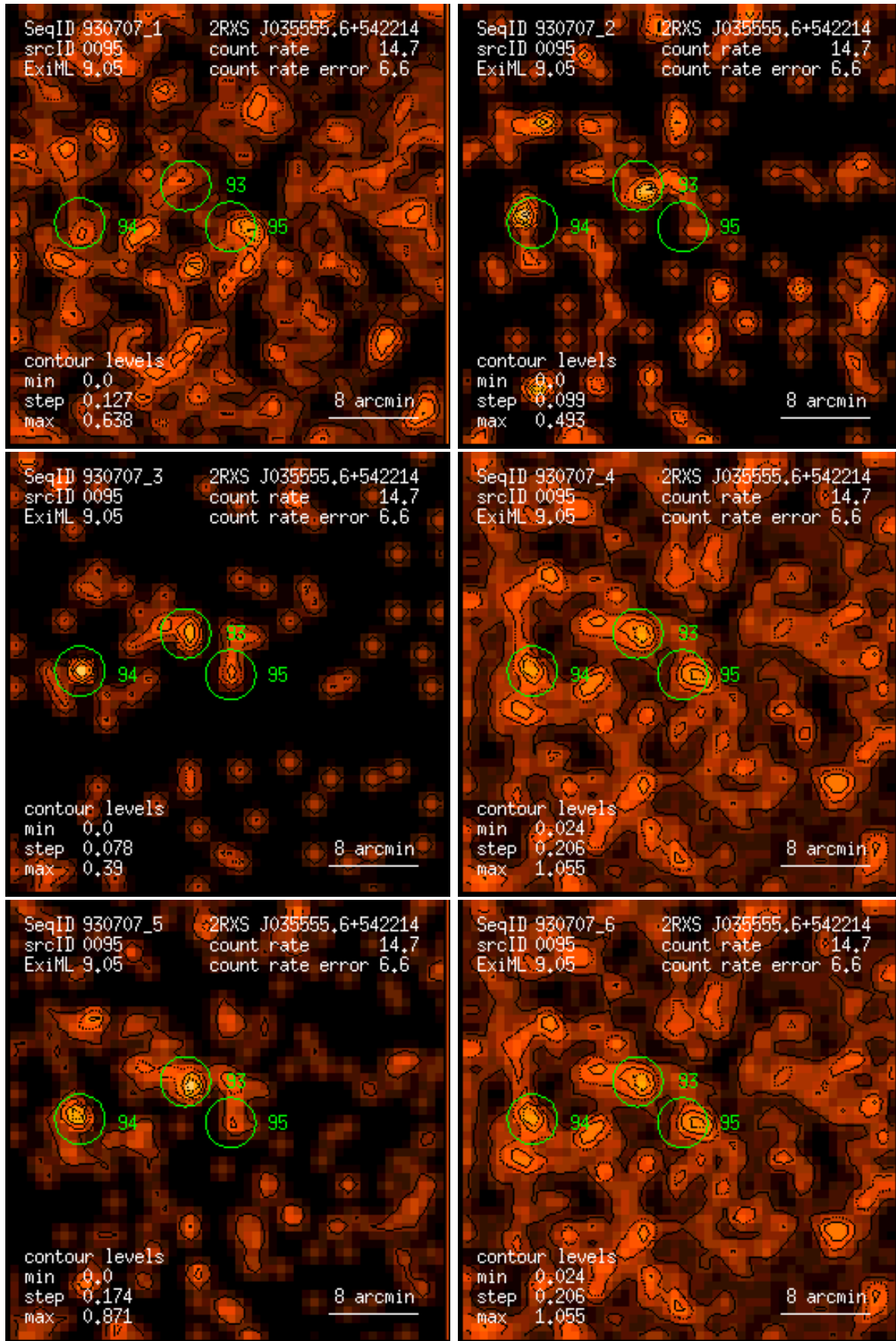
Figure 95: RASS 930707: detection 0095: band rate images, Gaussian filter: (1) PSPC channels 11 – 41, (2) 52 – 90, (3) 91 – 201, (4) 11 – 235, (5) 52 – 201, (6) 11 – 201. Broad band rates in counts/ks. Band rate contour levels in counts/ks/arcmin 2 .
