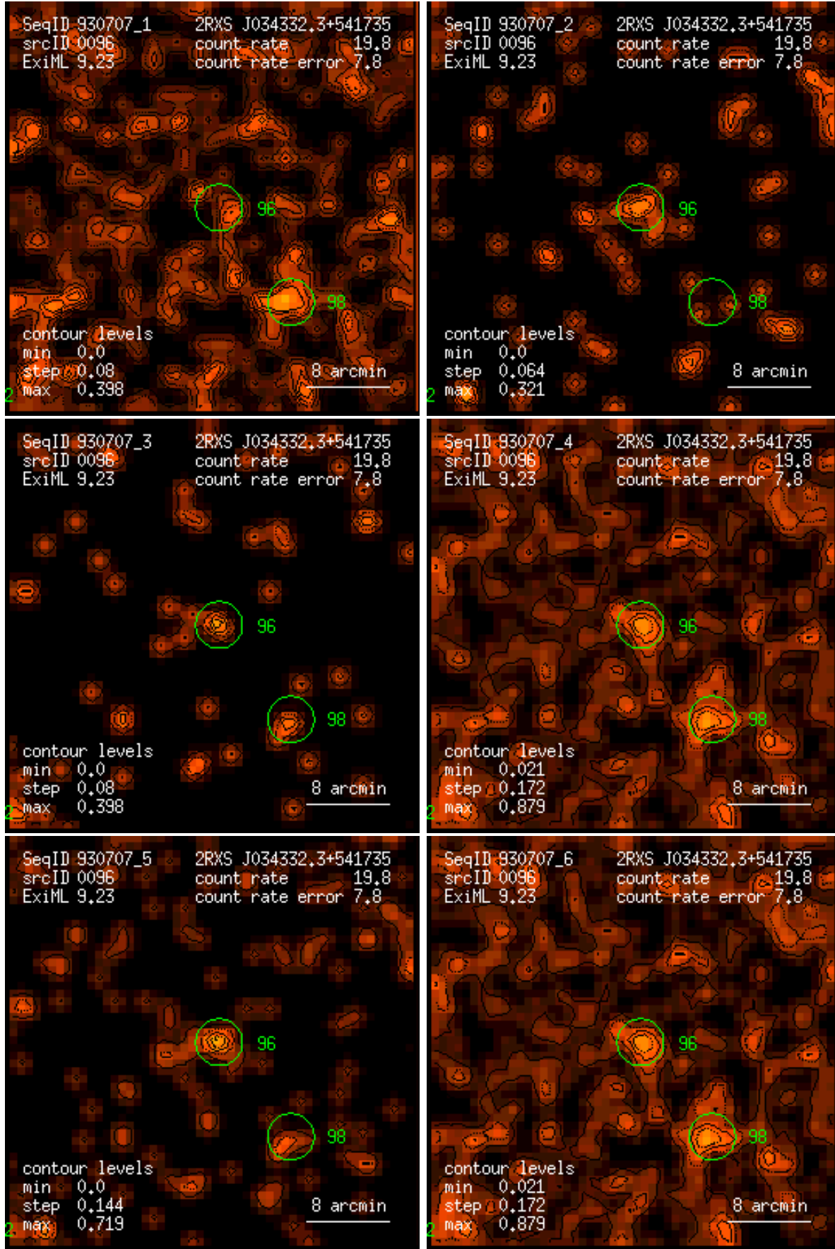
Figure 96: RASS 930707: detection 0096: band rate images, Gaussian filter: (1) PSPC channels 11 – 41, (2) 52 – 90, (3) 91 – 201, (4) 11 – 235, (5) 52 – 201, (6) 11 – 201. Broad band rates in counts/ks. Band rate contour levels in counts/ks/arcmin 2 .
