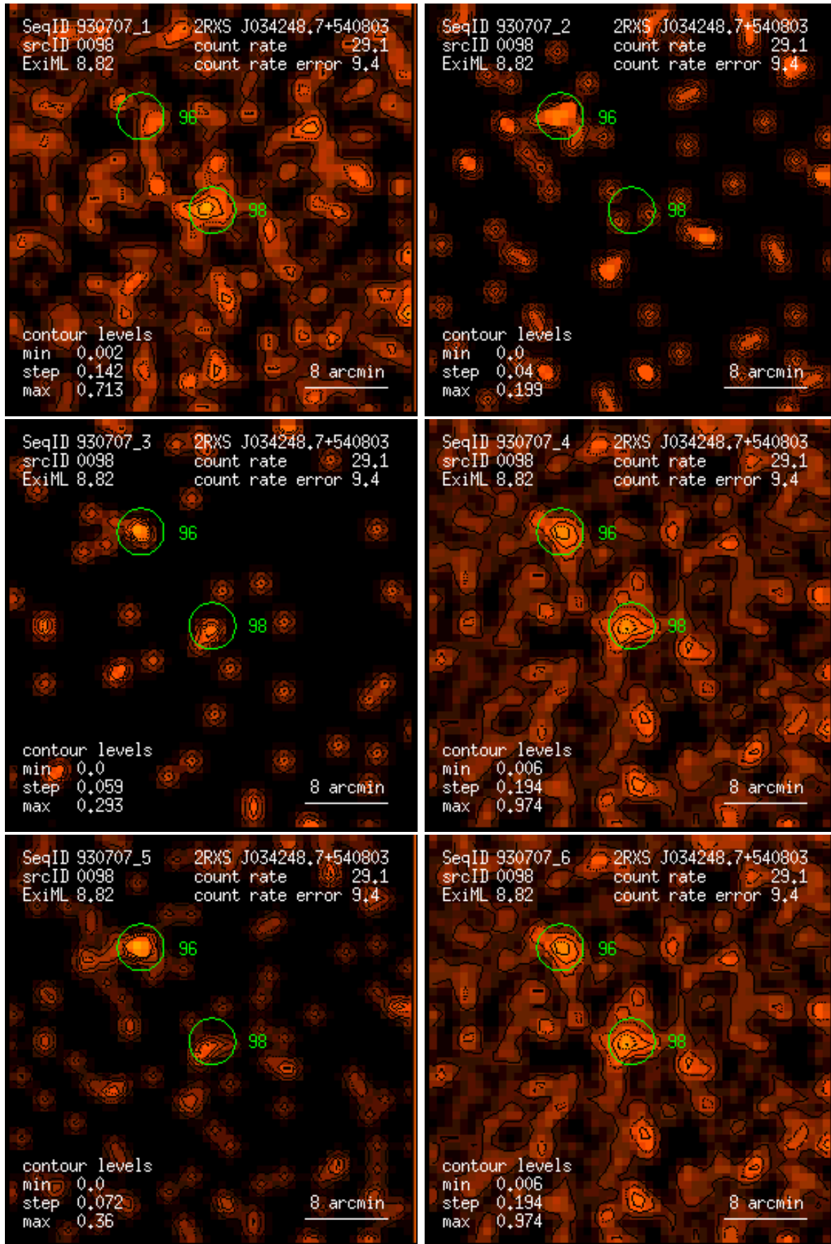
Figure 98: RASS 930707: detection 0098: band rate images, Gaussian filter: (1) PSPC channels 11 – 41, (2) 52 – 90, (3) 91 – 201, (4) 11 – 235, (5) 52 – 201, (6) 11 – 201. Broad band rates in counts/ks. Band rate contour levels in counts/ks/arcmin 2 .
